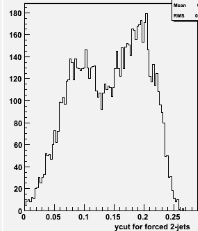
Ycut for 2-jets :w103223 e1a_e1csdu_o
