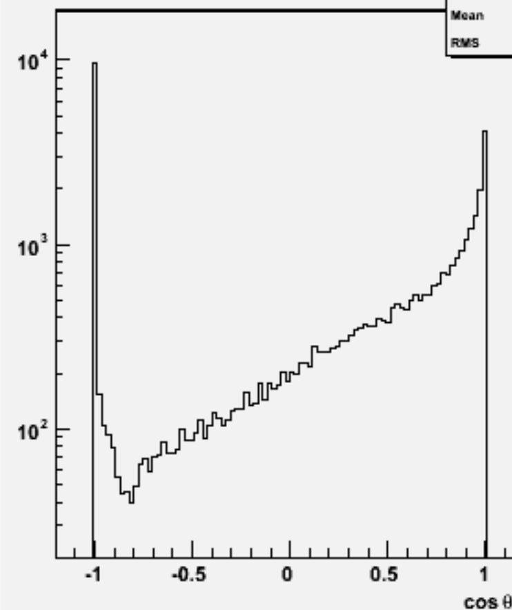
Jet cos \theta (All jets)w103223 e1a_e1csdu_o
