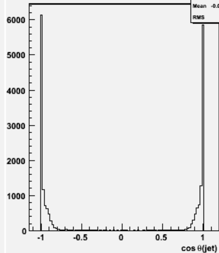
cos \theta for 2-jets :w103223 e1a_e1csdu_o
