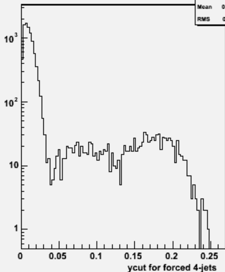
Ycut for 4-jets :w103223 e1a_e1csdu_o
