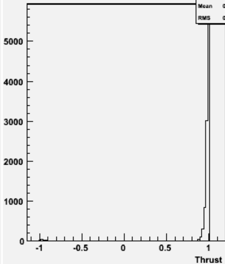
cos \Theta (thrust) w103223 e1a_e1csdu_o
