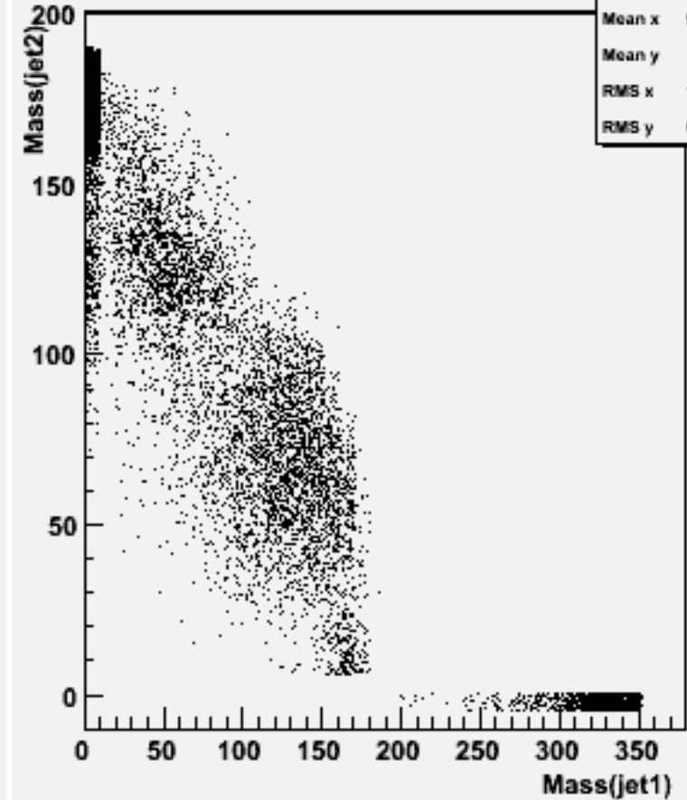
Jet mass for forced 2-jets : w103223 e1a_e1csdu_o
