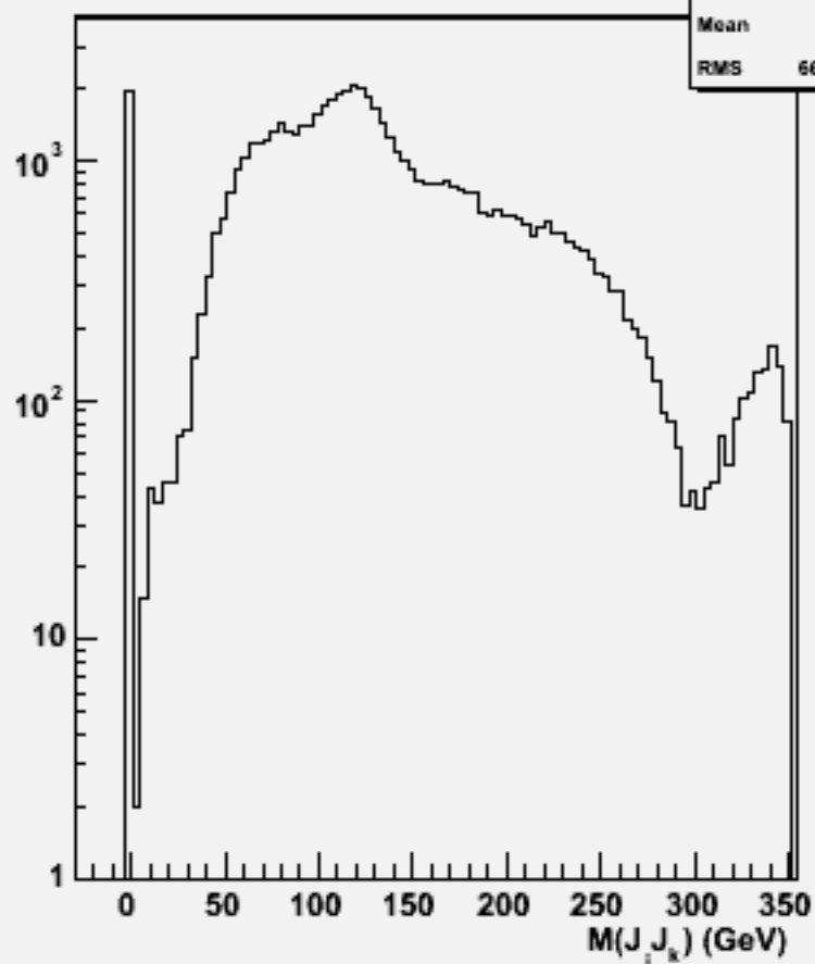
2jets mass(All comb)w103223 e1a_e1csdu_o
