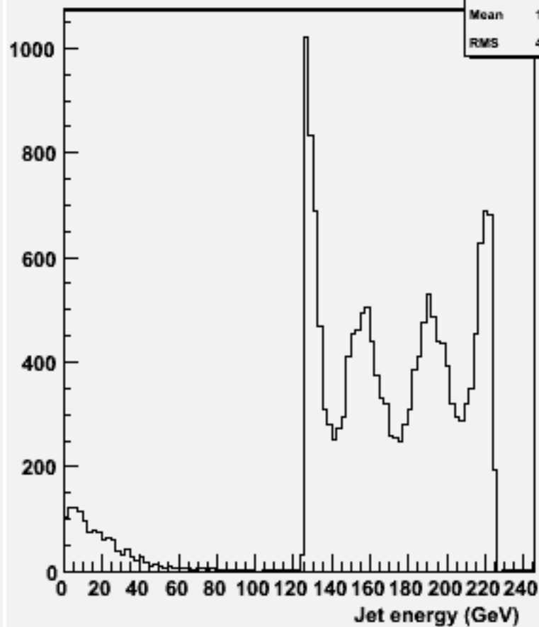
energy for 2-jets :w103223 e1a_e1csdu_o
