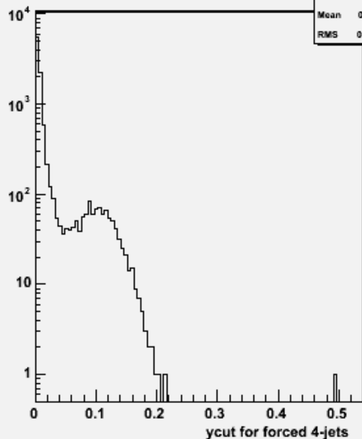
Ycut for 4-jets :w103221 e1a_e1cse3n3_o
