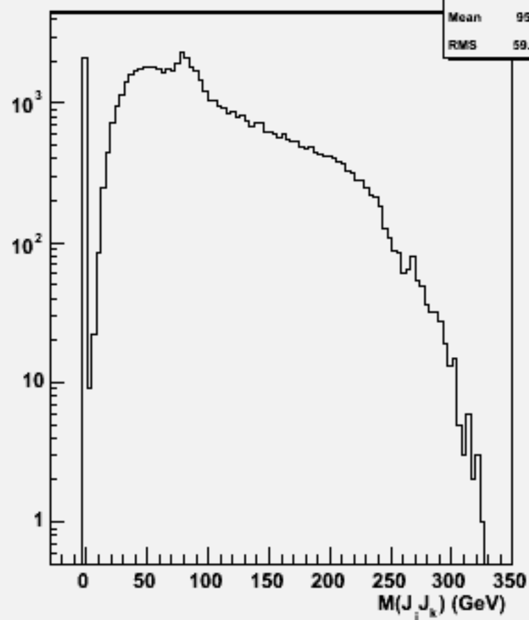
2jets mass(All comb)w103221 e1a_e1cse3n3_o
