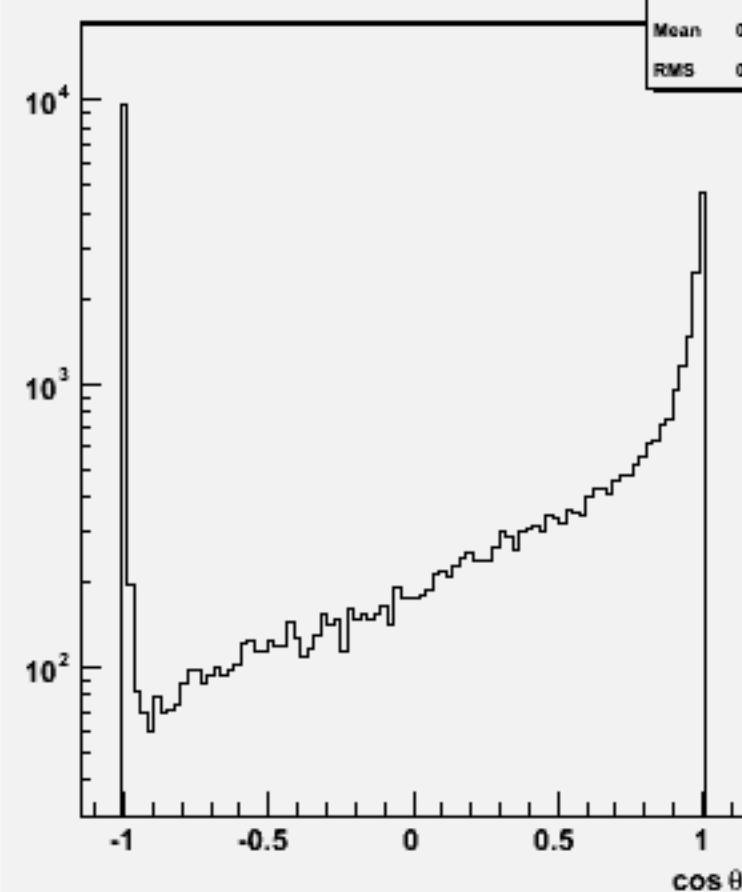
Jet cos \theta (All jets)w103221 e1a_e1cse3n3_o
