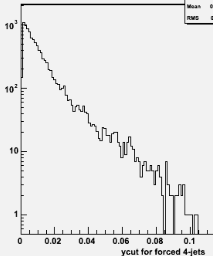
Ycut for 4-jets :w103218 e1a_e1cse3n3_o
