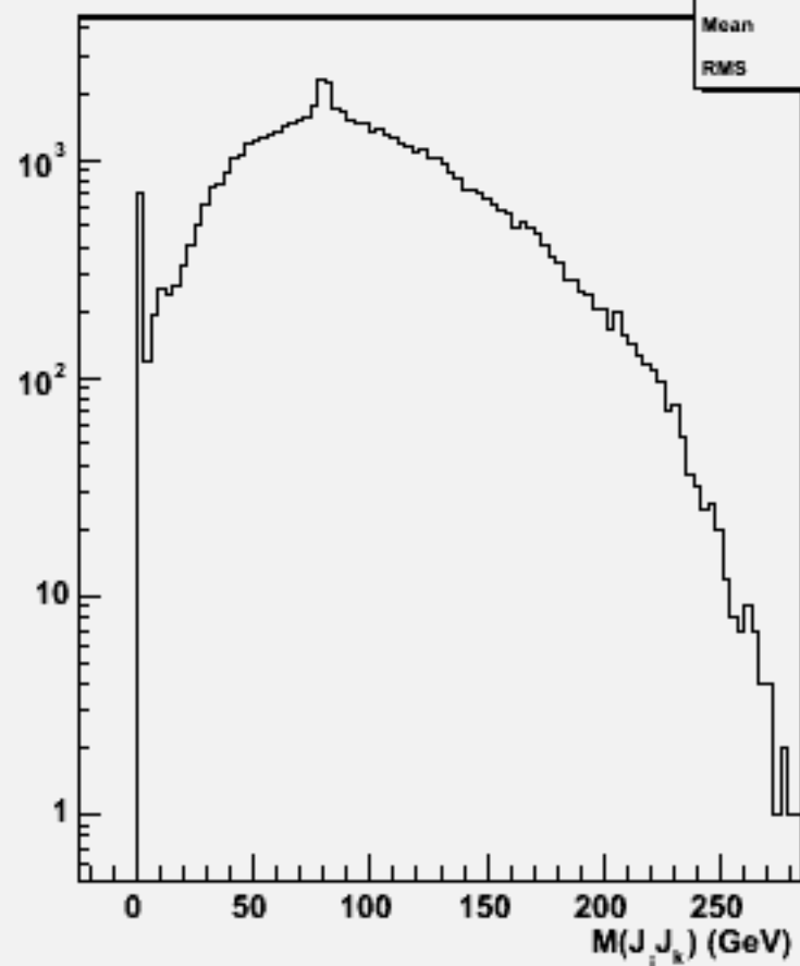
2jets mass(All comb)w103218 e1a_e1cse3n3_o
