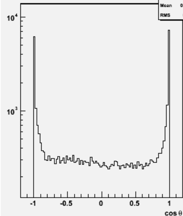
Jet cos \theta (All jets)w103218 e1a_e1cse3n3_o
