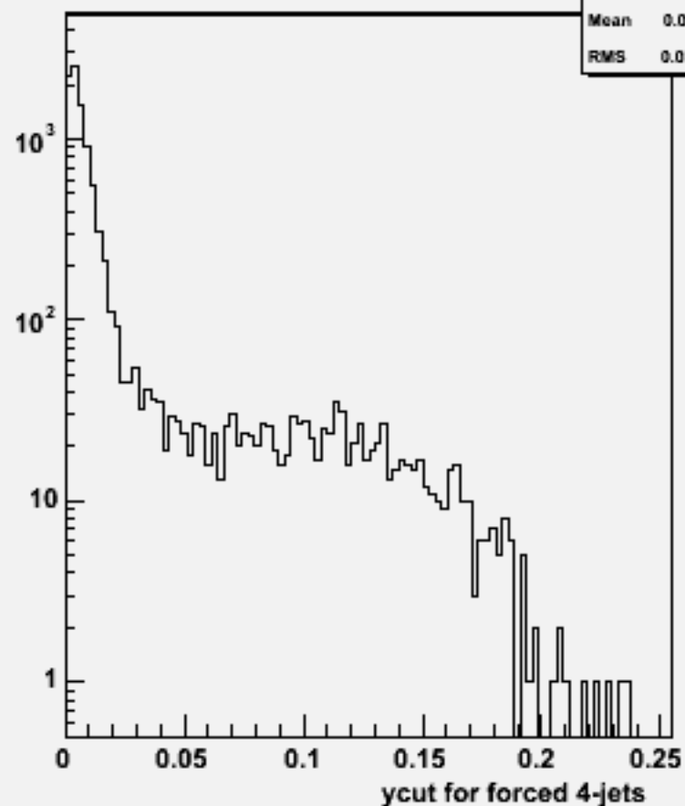
Ycut for 4-jets :w103217 e1a_e1cse2n2_o
