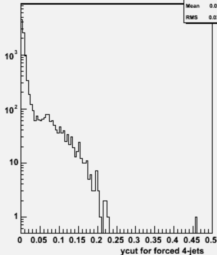
Ycut for 4-jets :w103213 e1a_e1cse1n1_o
