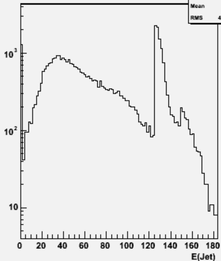
Jet energies(All jets)w103213 e1a_e1cse1n1_o
