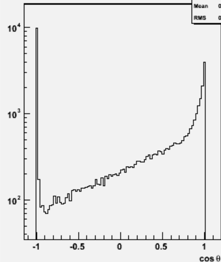
Jet cos \theta (All jets)w103213 e1a_e1cse1n1_o
