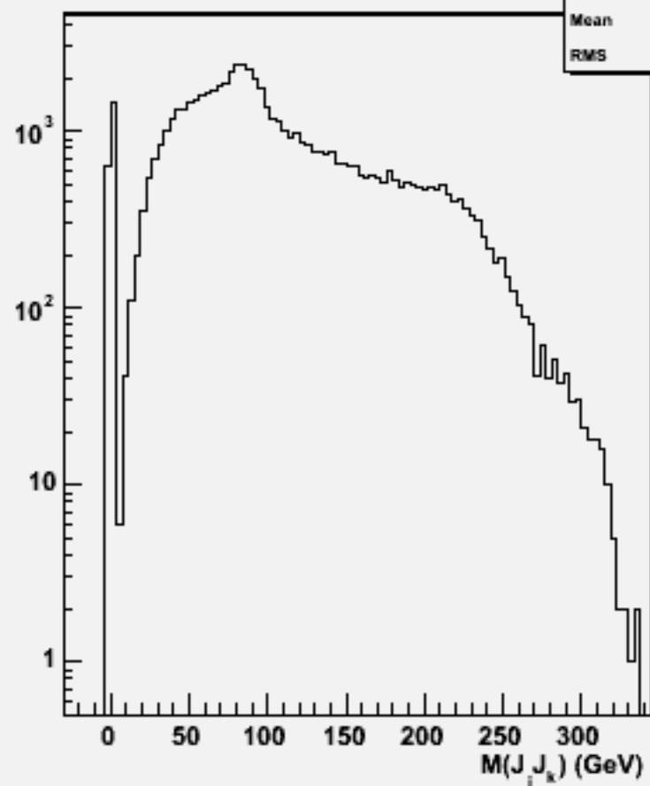
2jets mass(All comb)w103213 e1a_e1cse1n1_o
