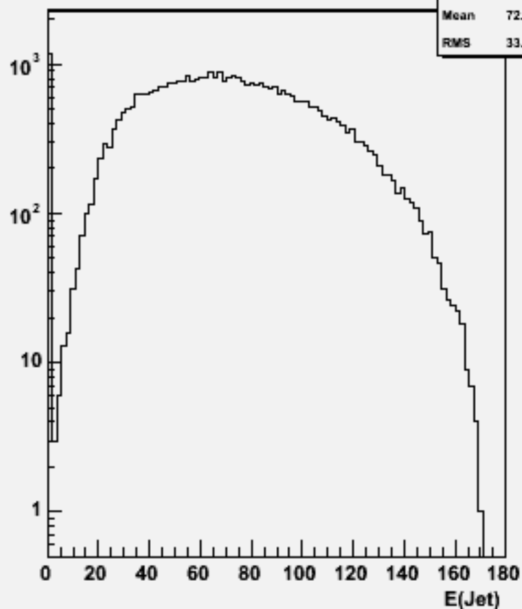
Jet energies(All jets)w103212 e1a_e1cse1n1_o
