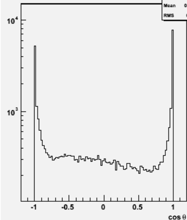
Jet cos \theta (All jets)w103212 e1a_e1cse1n1_o
