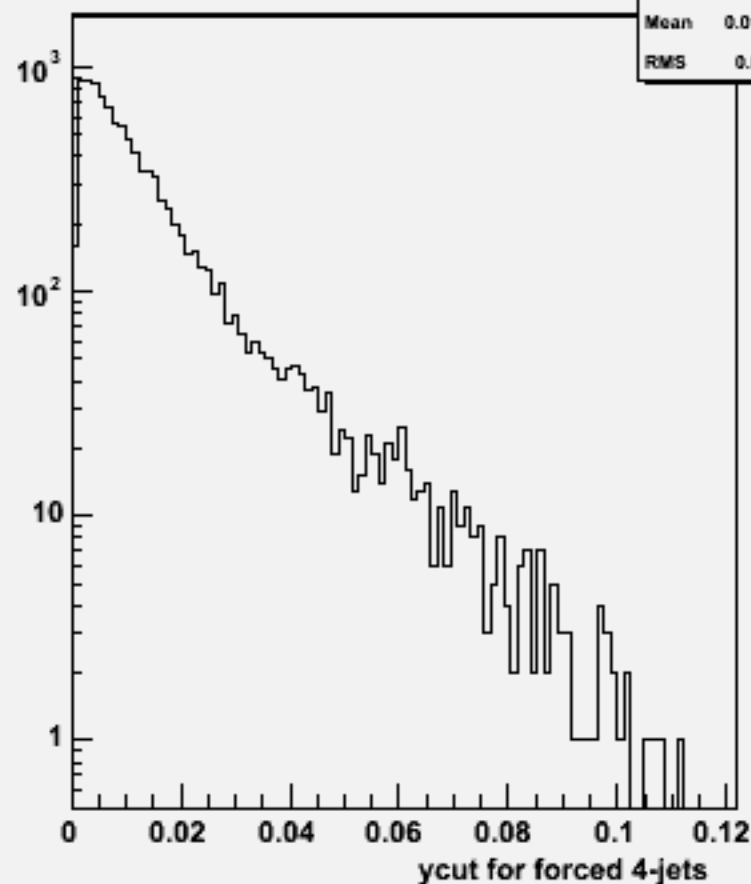
Ycut for 4-jets :w103212 e1a_e1cse1n1_o
