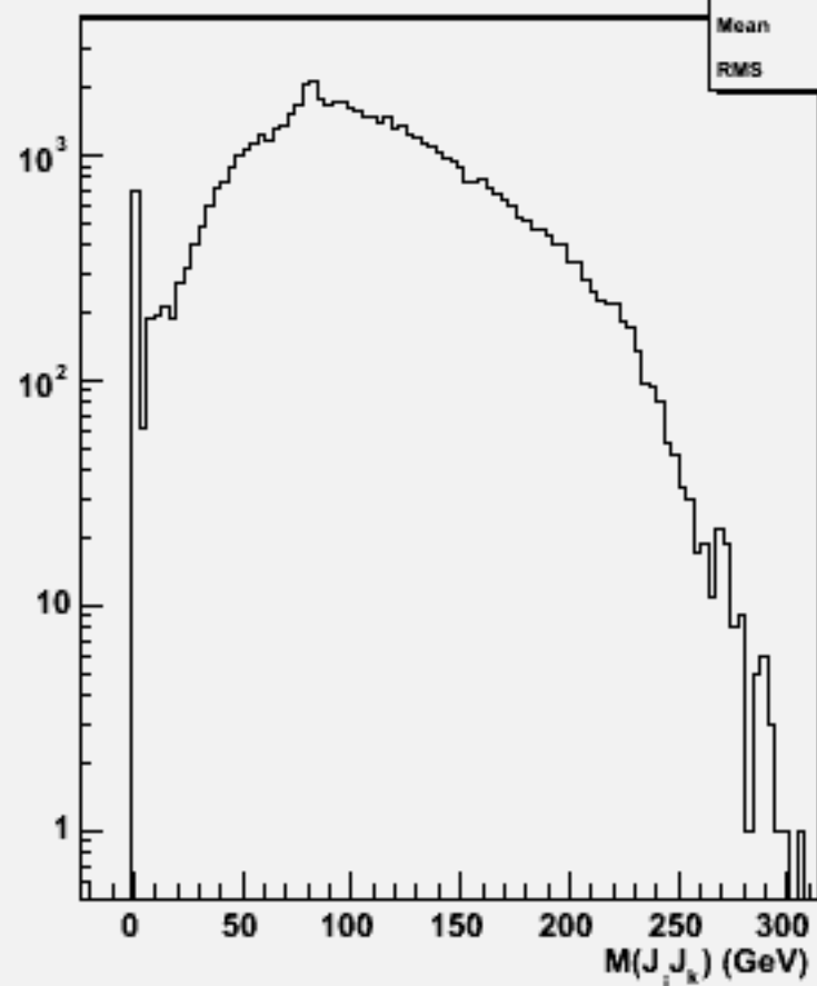
2jets mass(All comb)w103212 e1a_e1cse1n1_o
