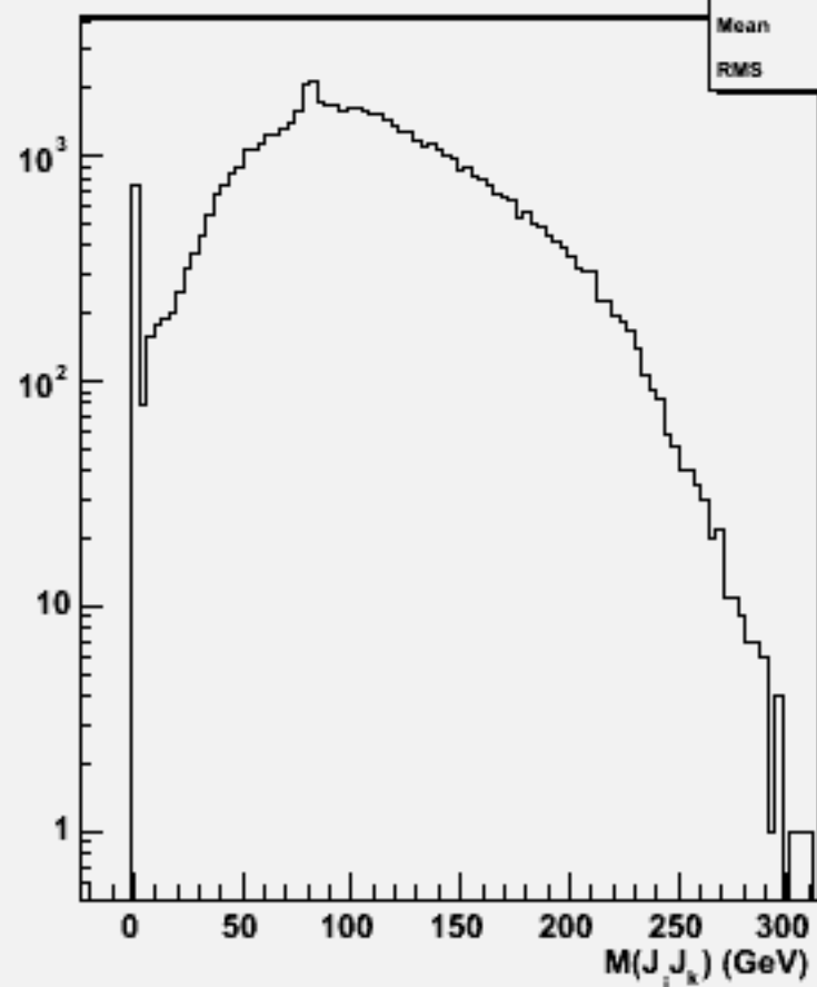
2jets mass(All comb)w103210 e1a_e1cse1n1_o
