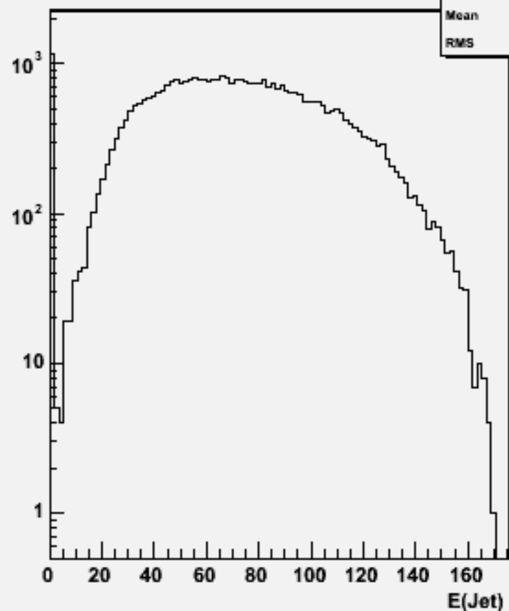
Jet energies(All jets)w103210 e1a_e1cse1n1_o
