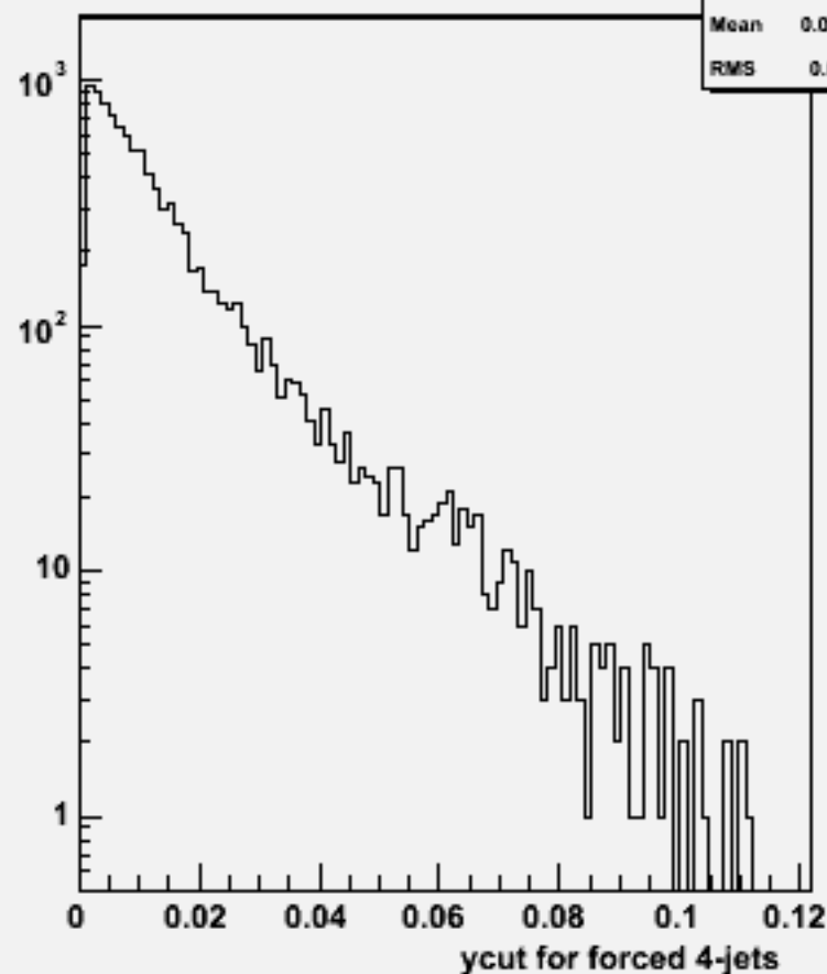
Ycut for 4-jets :w103210 e1a_e1cse1n1_o
