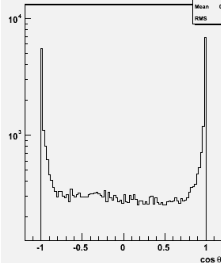
Jet cos \theta (All jets)w103210 e1a_e1cse1n1_o
