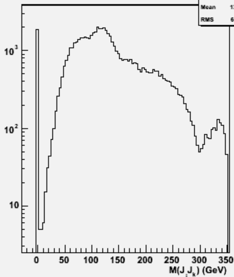
2jets mass(All comb)w103209 e1a_e1udsc_o
