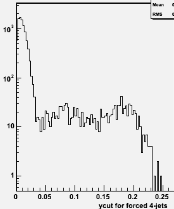
Ycut for 4-jets :w103209 e1a_e1udsc_o
