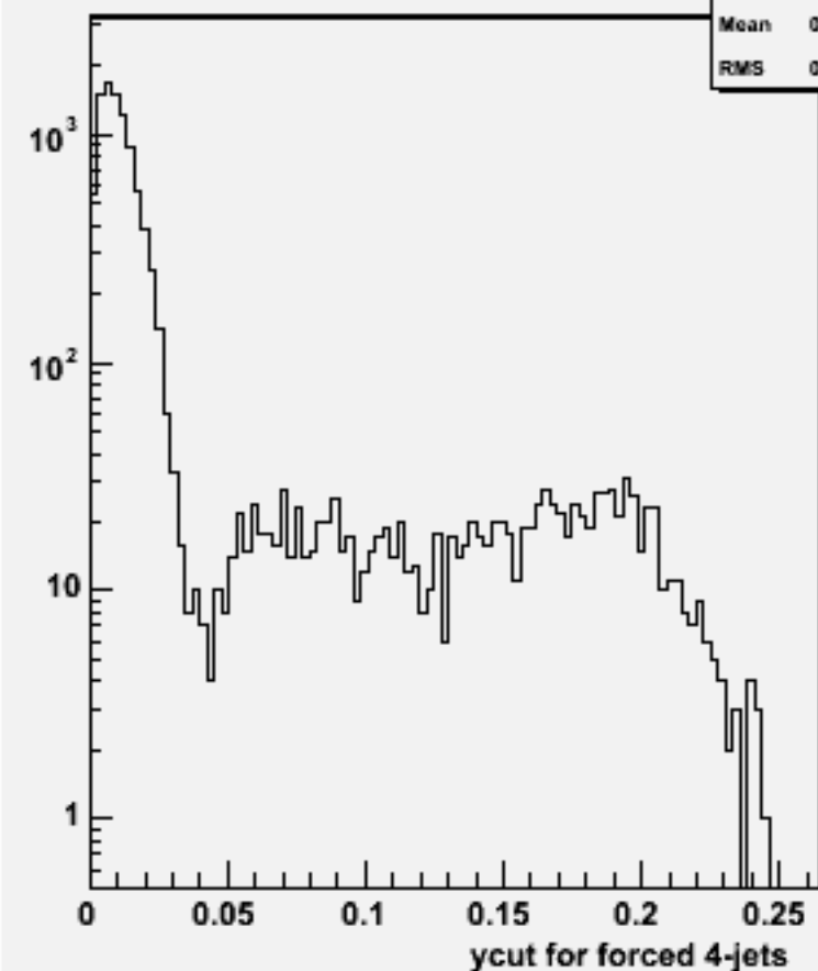
Ycut for 4-jets :w103207 e1a_e1udsc_o
