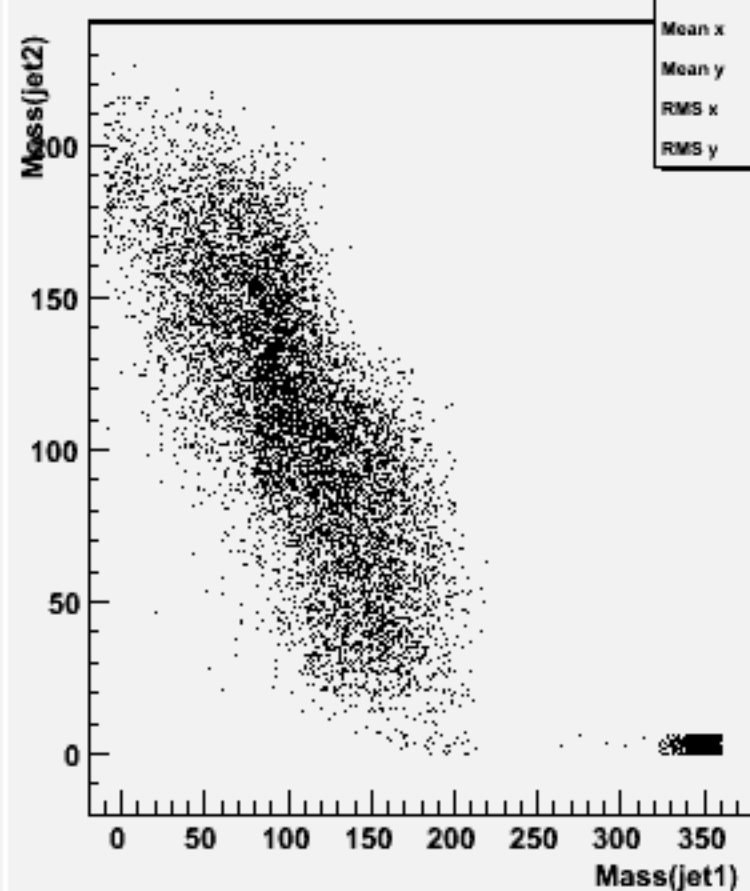
Jet mass for forced 2-jets : w103204 e1a_e1uddu_o
