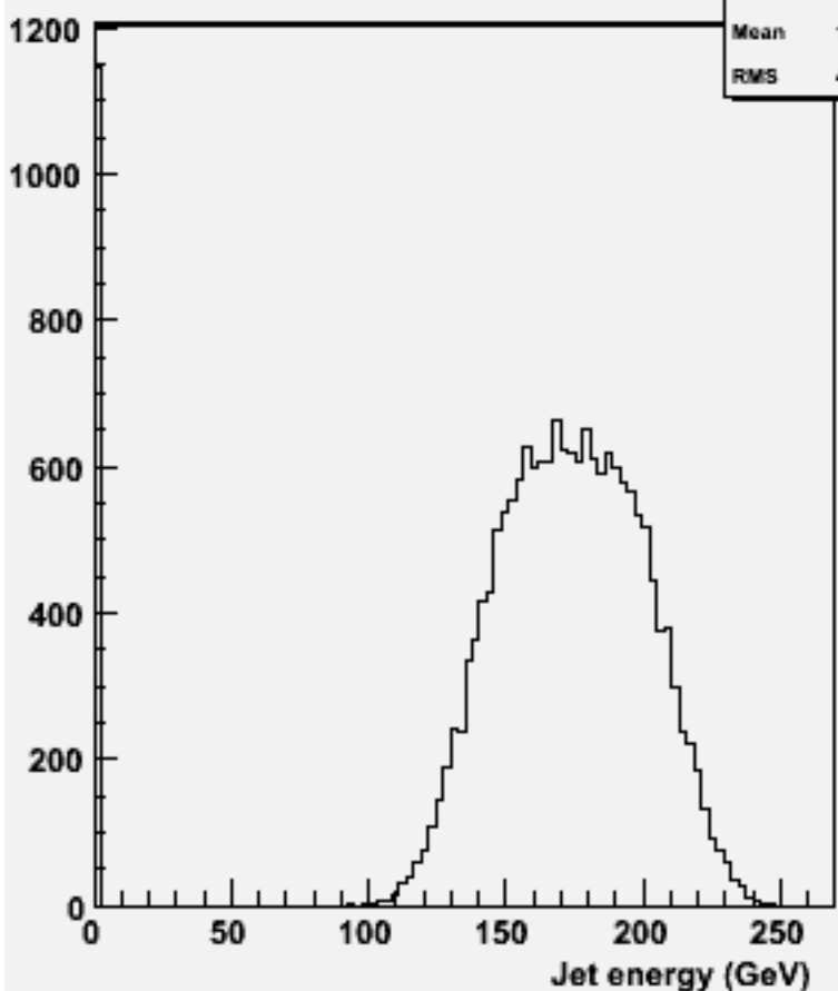
energy for 2-jets :w103204 e1a_e1uddu_o
