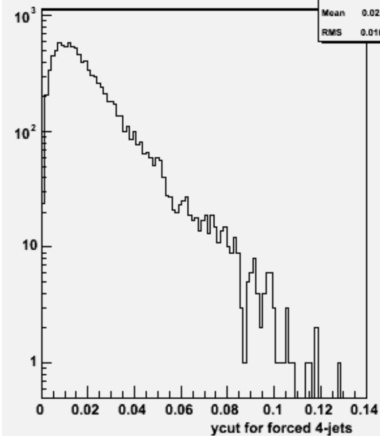
Ycut for 4-jets :w103204 e1a_e1uddu_o
