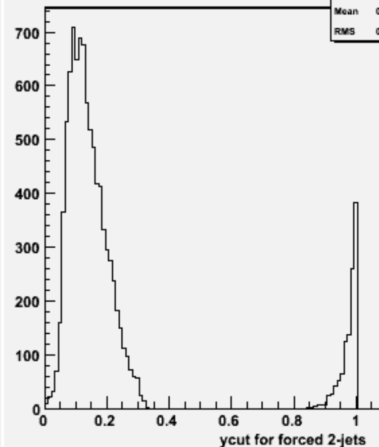
Ycut for 2-jets :w103204 e1a_e1uddu_o
