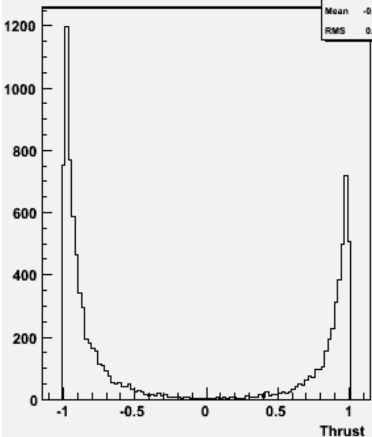
cos \Theta (thrust) w103204 e1a_e1uddu_o
