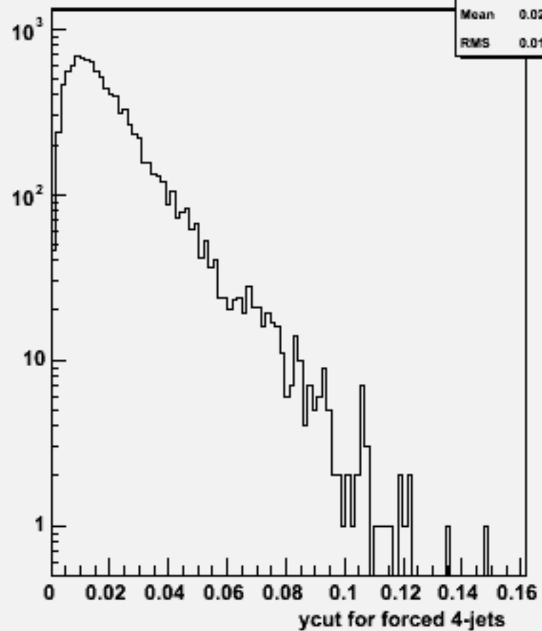
Ycut for 4-jets :w103202 e1a_e1uddu_o
