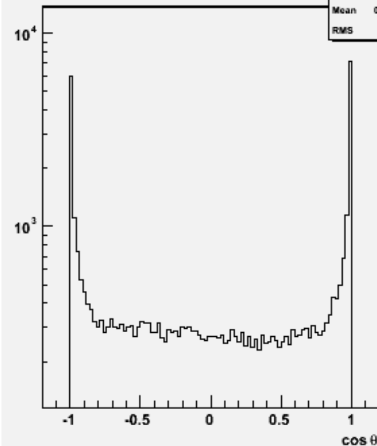
Jet cos \theta (All jets)w103198 e1a_e1ude3n3_o
