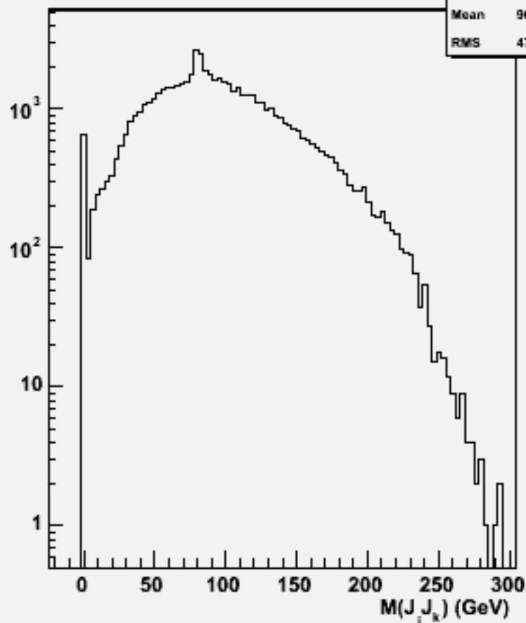
2jets mass(All comb)w103198 e1a_e1ude3n3_o
