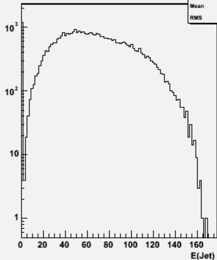
Jet energies(All jets)w103198 e1a_e1ude3n3_o
