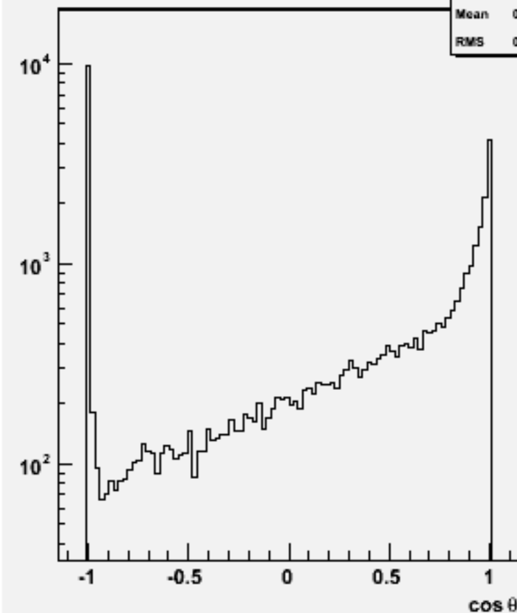
Jet cos \theta (All jets)w103197 e1a_e1ude2n2_o
