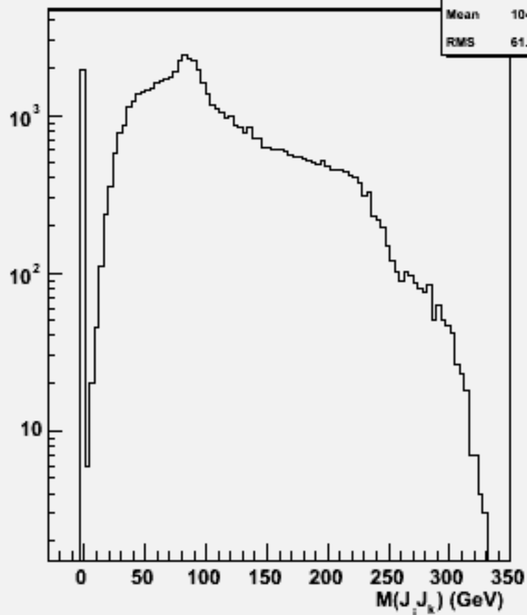
2jets mass(All comb)w103197 e1a_e1ude2n2_o
