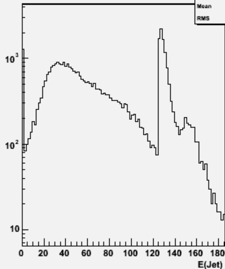
Jet energies(All jets)w103197 e1a_e1ude2n2_o
