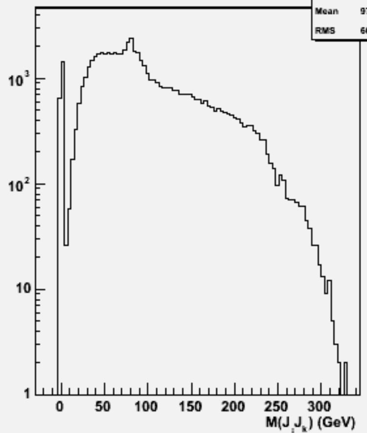
2jets mass(All comb)w103189 e1a_e1n3e3sc_o
