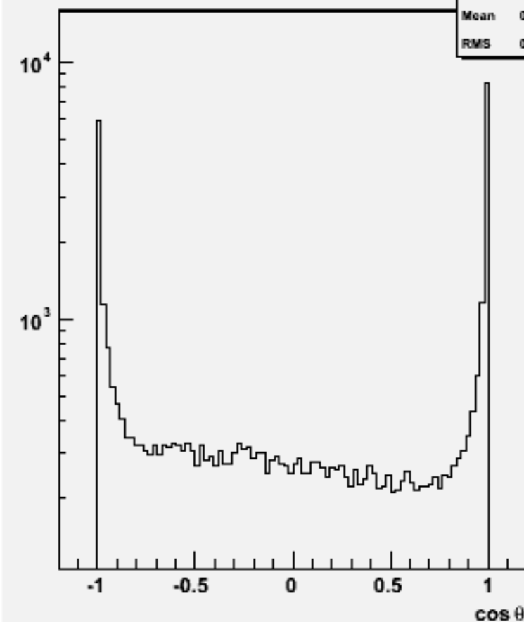
Jet cos \theta (All jets)w103188 e1a_e1n3e3sc_o
