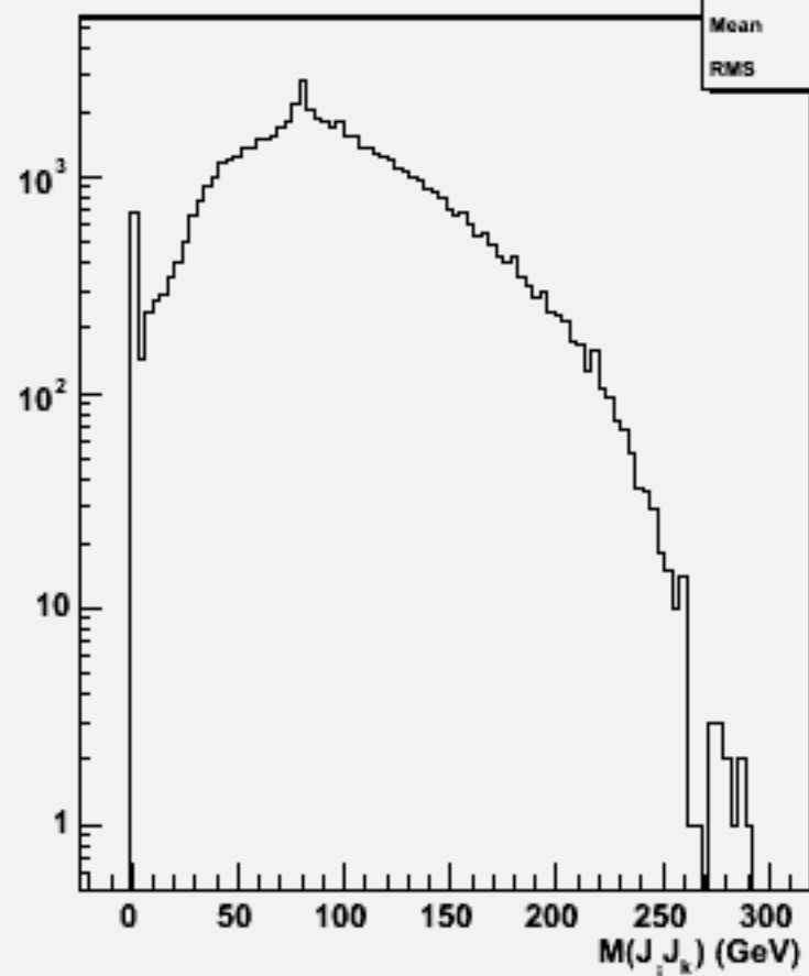
2jets mass(All comb)w103188 e1a_e1n3e3sc_o
