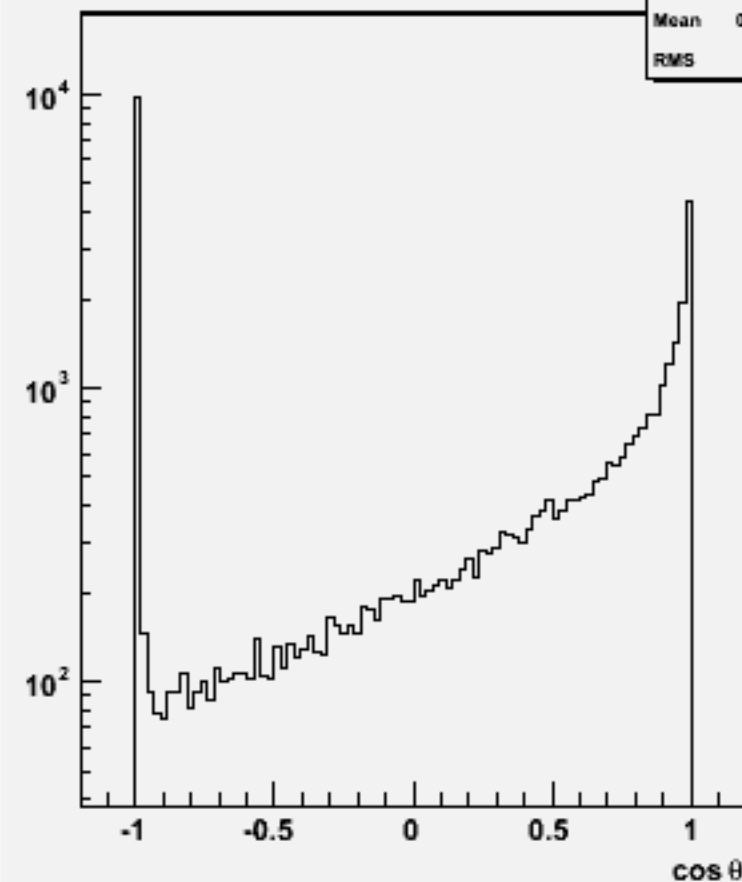
Jet cos \theta (All jets)w103187 e1a_e1n3e3sc_o
