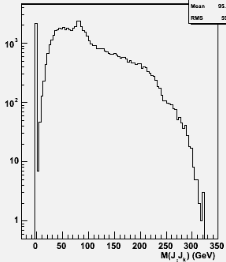
2jets mass(All comb)w103187 e1a_e1n3e3sc_o
