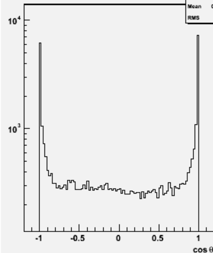
Jet cos \theta (All jets)w103186 e1a_e1n3e3sc_o
