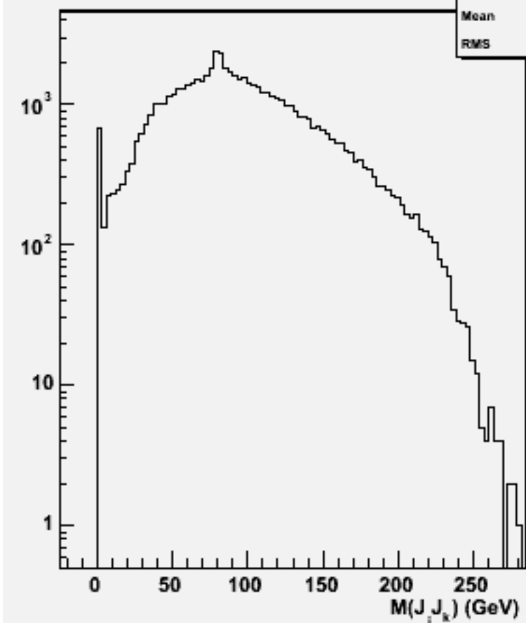
2jets mass(All comb)w103186 e1a_e1n3e3sc_o
