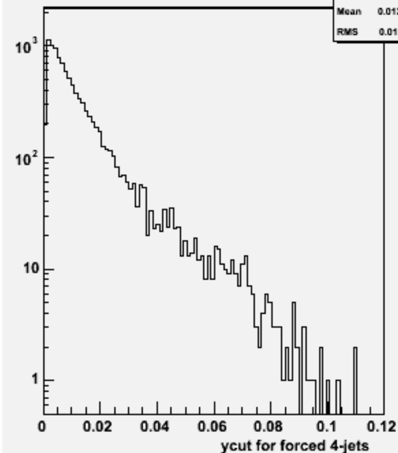
Ycut for 4-jets :w103186 e1a_e1n3e3sc_o
