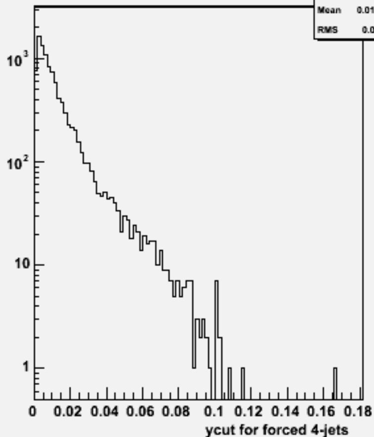
Ycut for 4-jets :w103182 e1a_e1n3e3du_o
