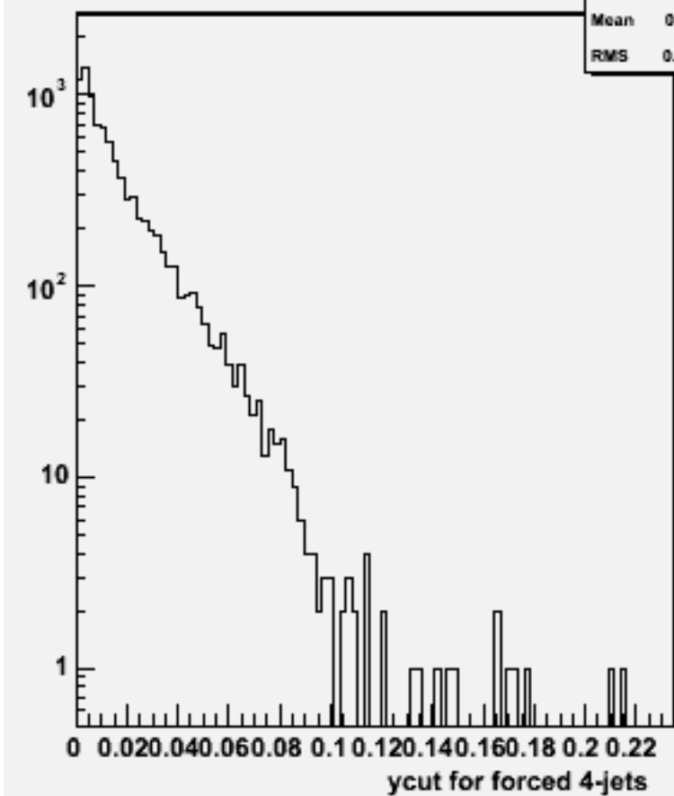
Ycut for 4-jets :w103180 e1a_e1n3e3e3n3_o
