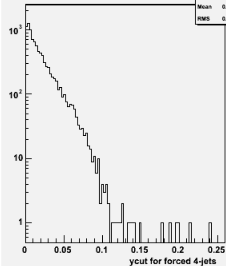
Ycut for 4-jets :w103176 e1a_e1n3e3e2n2_o
