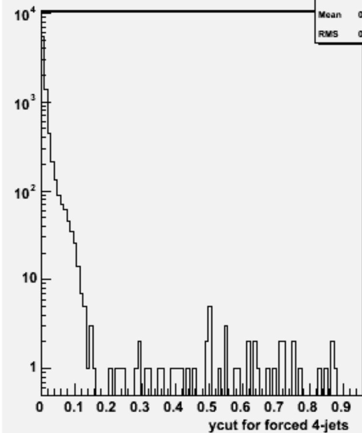
Ycut for 4-jets :w103175 e1a_e1n3e3e2n2_o
