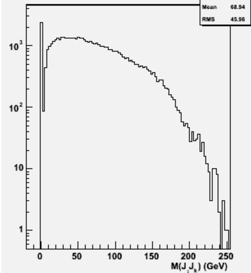
2jets mass(All comb)w103174 e1a_e1n3e3e2n2_o
