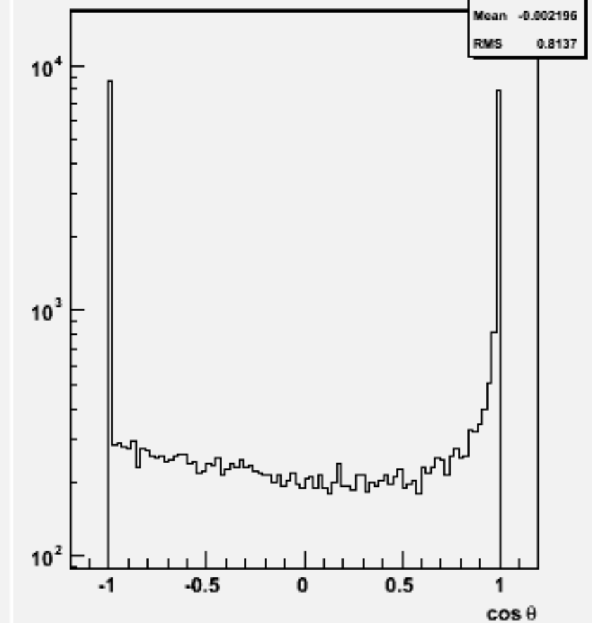
Jet cos \theta (All jets)w103174 e1a_e1n3e3e2n2_o
