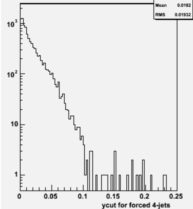
Ycut for 4-jets :w103174 e1a_e1n3e3e2n2_o
