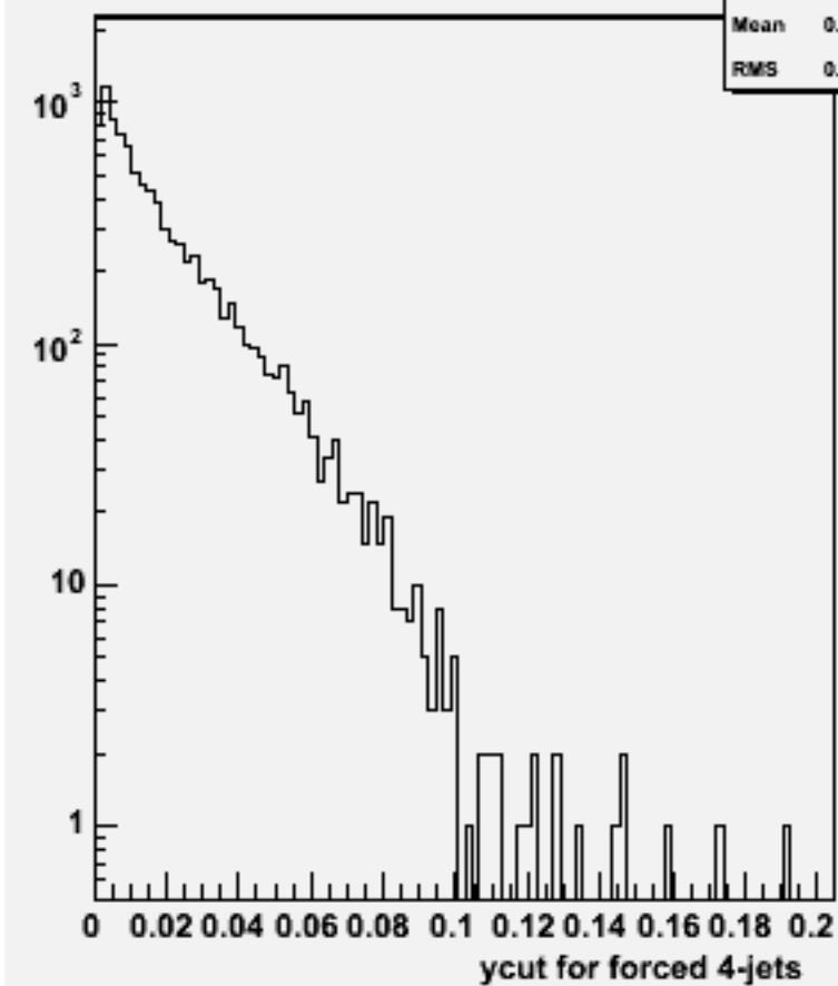
Ycut for 4-jets :w103172 e1a_e1n3e3e1n1_o
