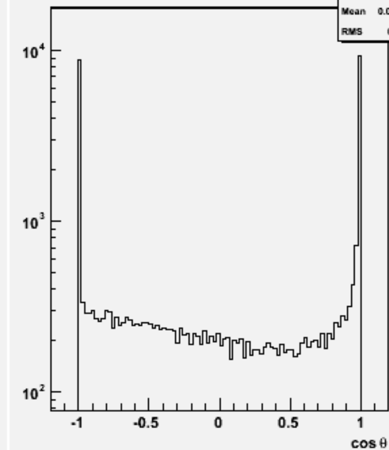
Jet cos \theta (All jets)w103172 e1a_e1n3e3e1n1_o
