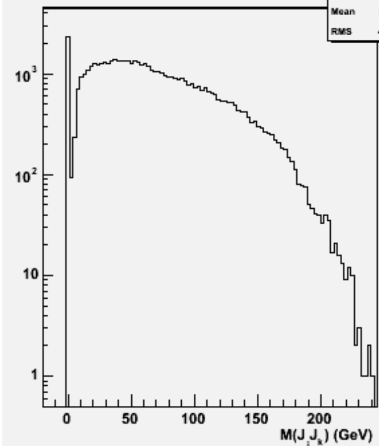
2jets mass(All comb)w103172 e1a_e1n3e3e1n1_o
