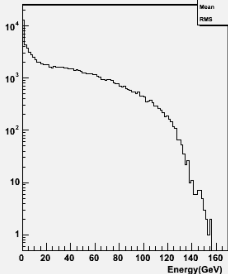
Particle Energy : w103172 e1a_e1n3e3e1n1_o
