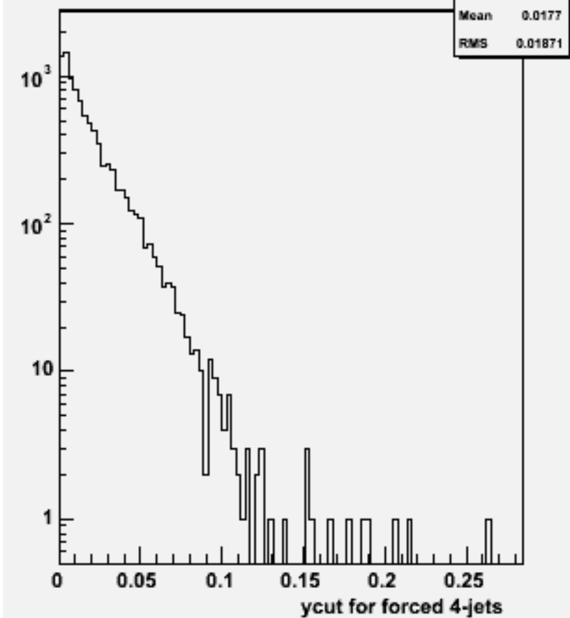
Ycut for 4-jets :w103170 e1a_e1n3e3e1n1_o
