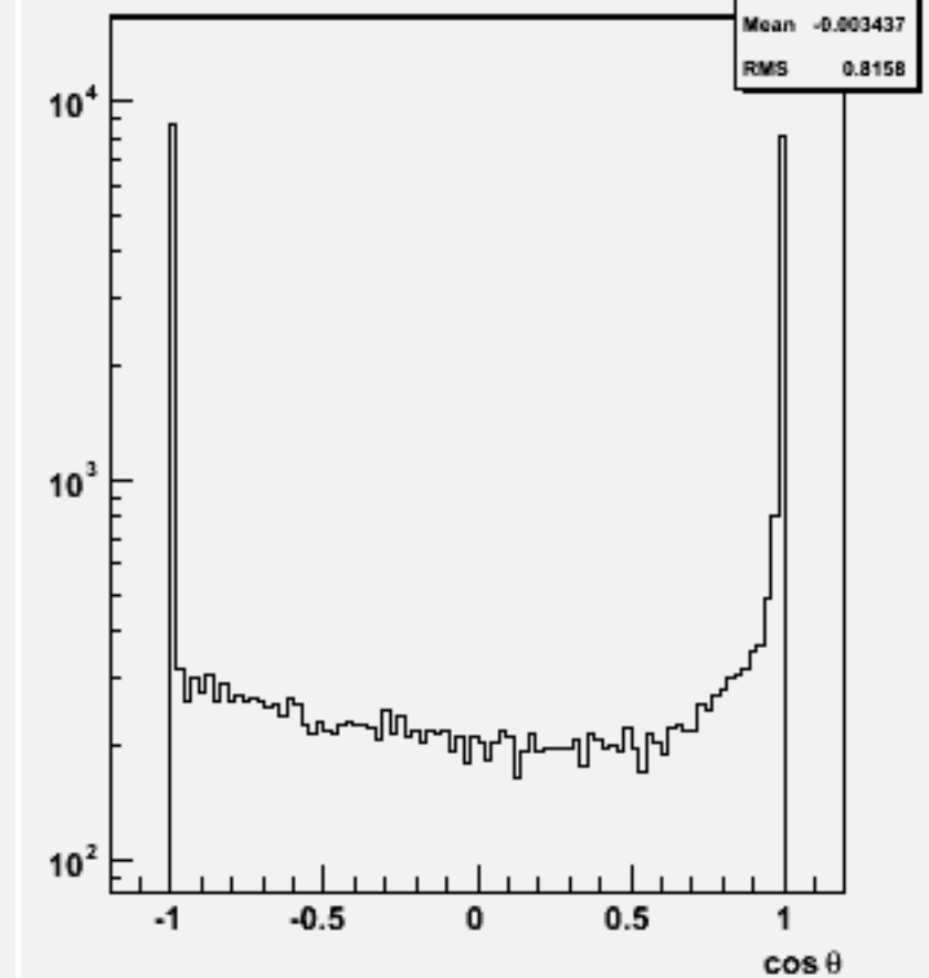
Jet cos \theta (All jets)w103170 e1a_e1n3e3e1n1_o
