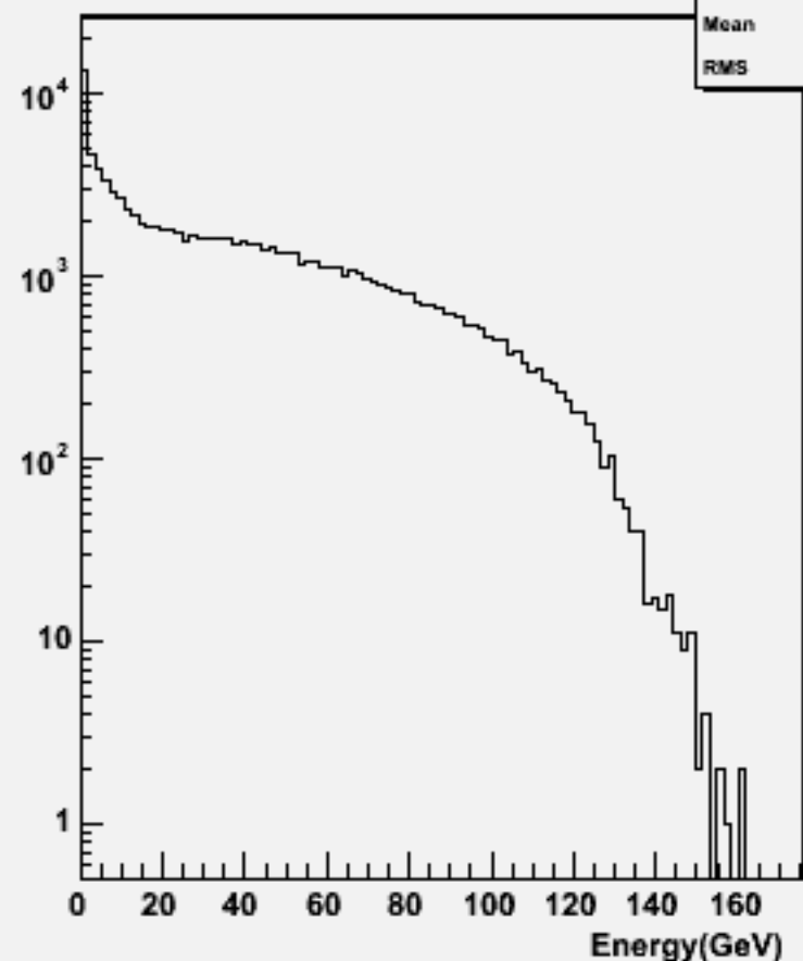
Particle Energy : w103170 e1a_e1n3e3e1n1_o
