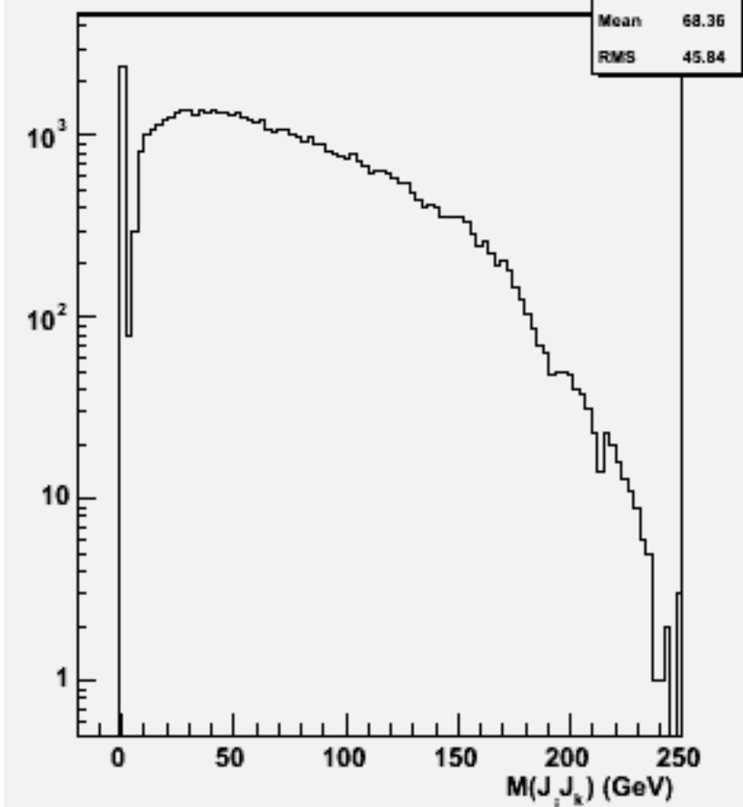
2jets mass(All comb)w103170 e1a_e1n3e3e1n1_o
