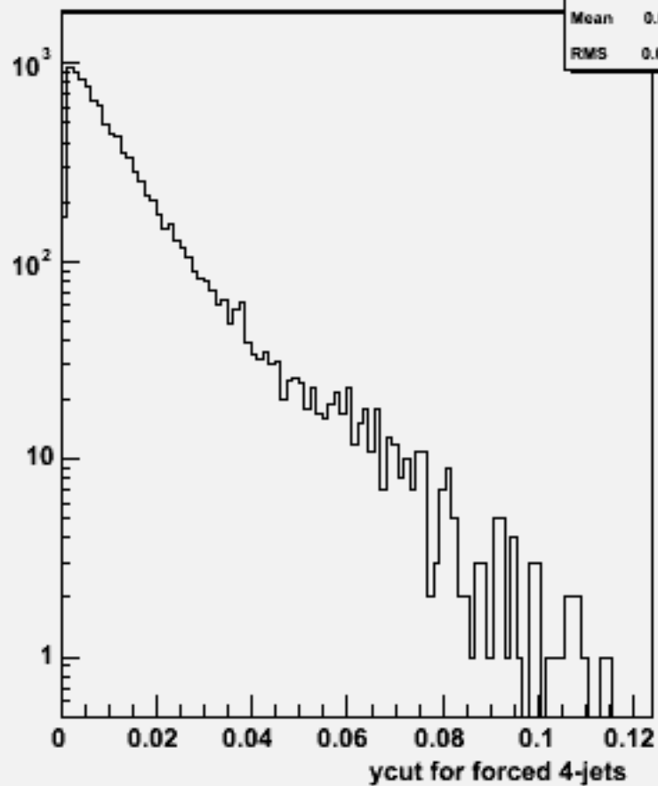
Ycut for 4-jets :w103168 e1a_e1n2e2sc_o
