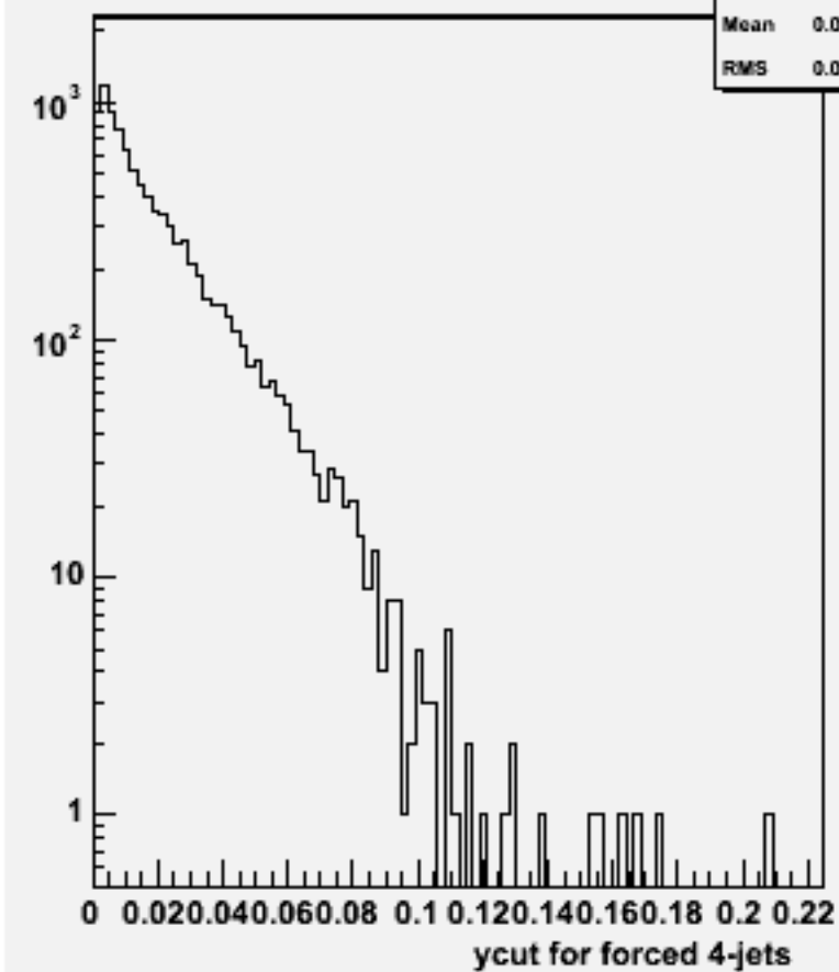
Ycut for 4-jets :w103160 e1a_e1n2e2e3n3_o
