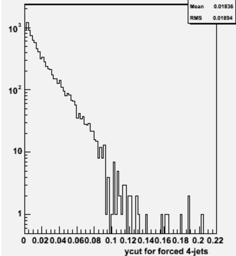
Ycut for 4-jets :w103158 e1a_e1n2e2e3n3_o
