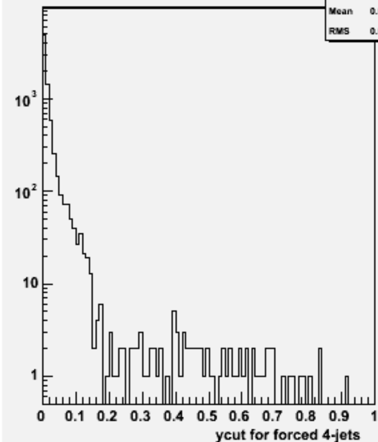
Ycut for 4-jets :w103157 e1a_e1n2e2e2n2_o
