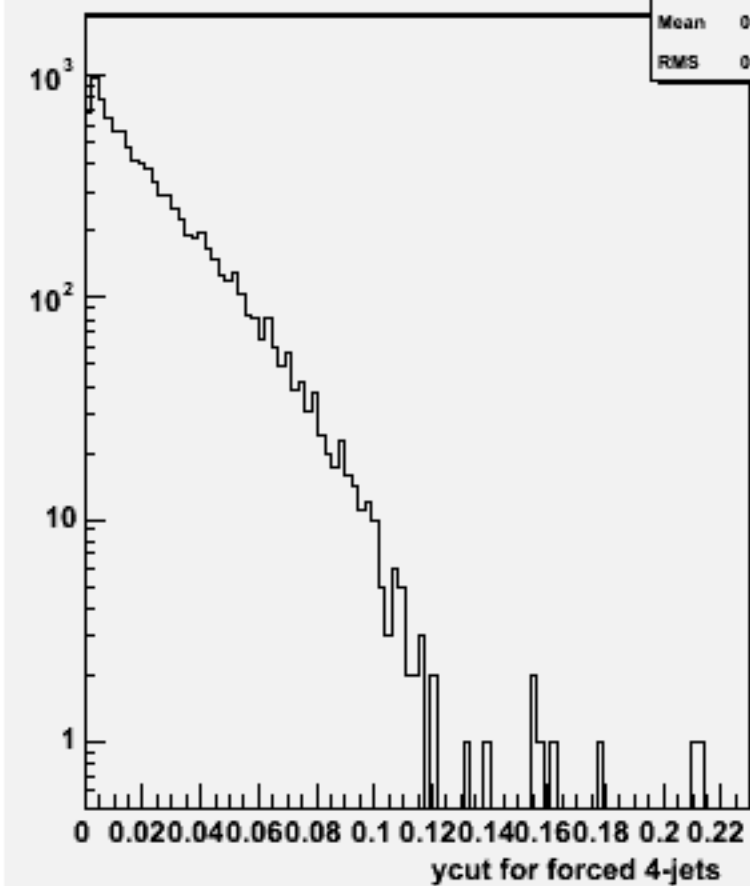
Ycut for 4-jets :w103156 e1a_e1n2e2e2n2_o
