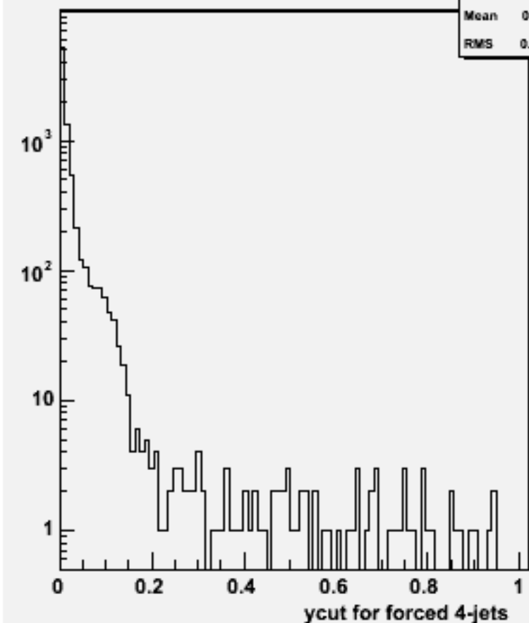
Ycut for 4-jets :w103155 e1a_e1n2e2e2n2_o
