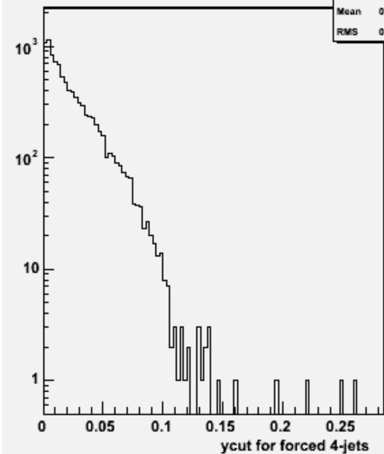
Ycut for 4-jets :w103154 e1a_e1n2e2e2n2_o
