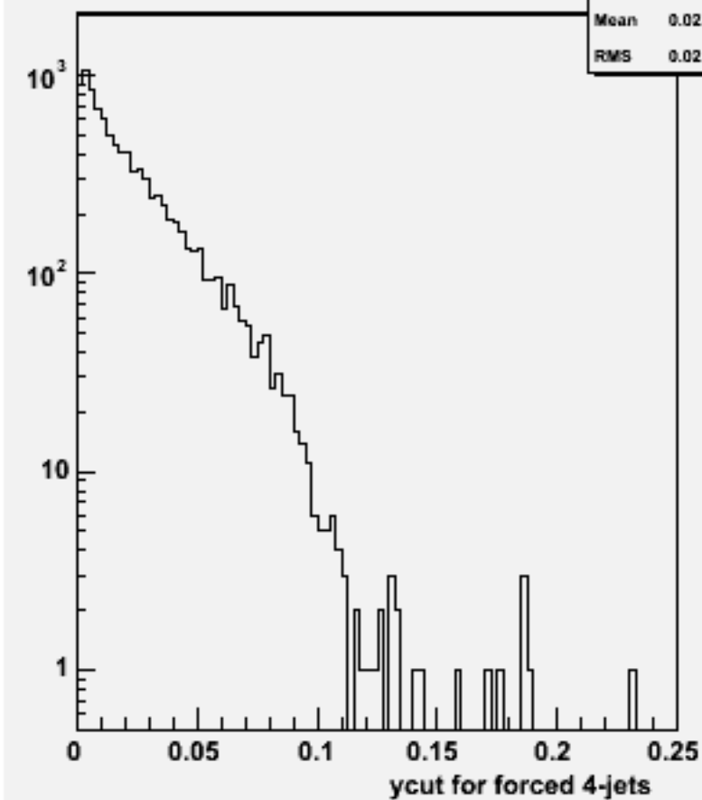
Ycut for 4-jets :w103150 e1a_e1n2e2e1n1_o
