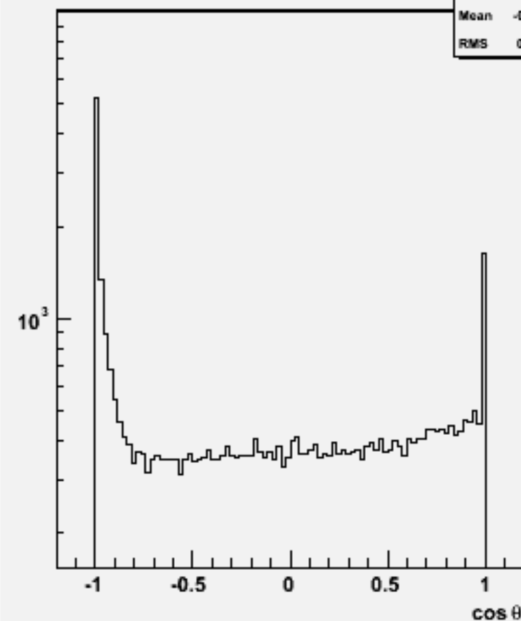
Jet cos \theta (All jets)w103146 e1a_n1bbsc_o
