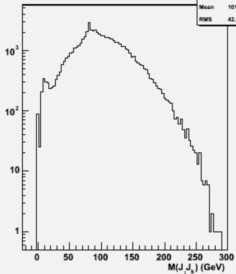
2jets mass(All comb)w103146 e1a_n1bbsc_o
