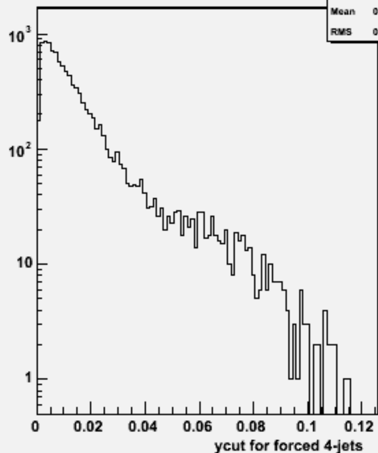
Ycut for 4-jets :w103146 e1a_n1bbsc_o
