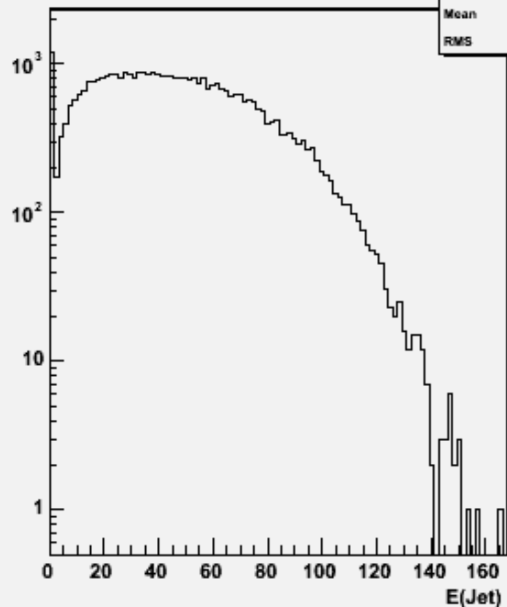
Jet energies(All jets)w103138 e1a_n1bbe3n3_o
