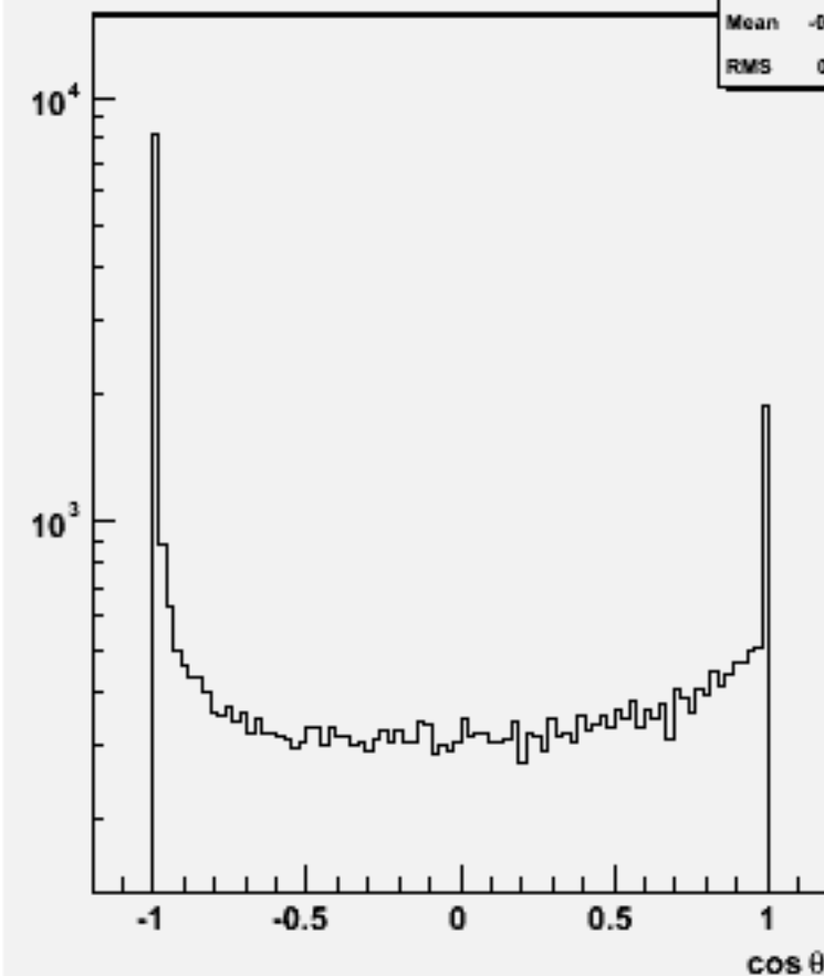
Jet cos \theta (All jets)w103138 e1a_n1bbe3n3_o
