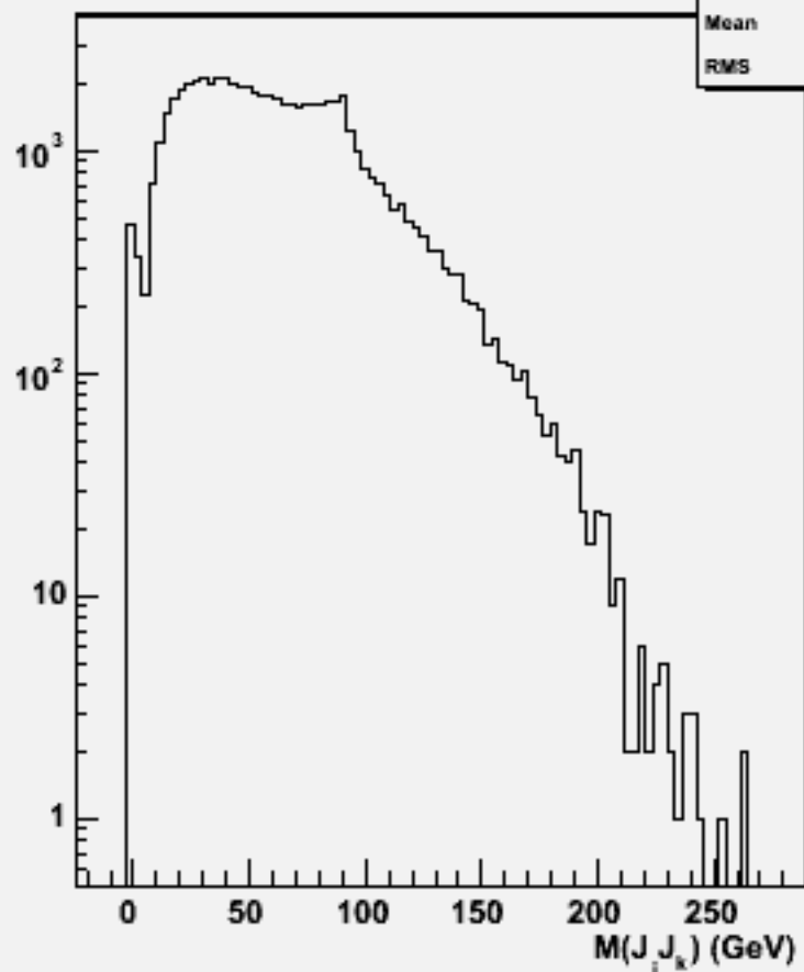
2jets mass(All comb)w103138 e1a_n1bbe3n3_o
