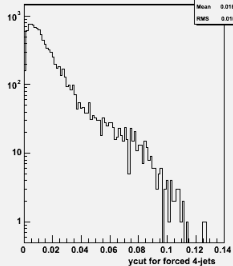
Ycut for 4-jets :w103126 e1a_n1sssc_o
