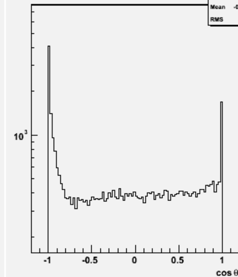
Jet cos \theta (All jets)w103126 e1a_n1sssc_o
