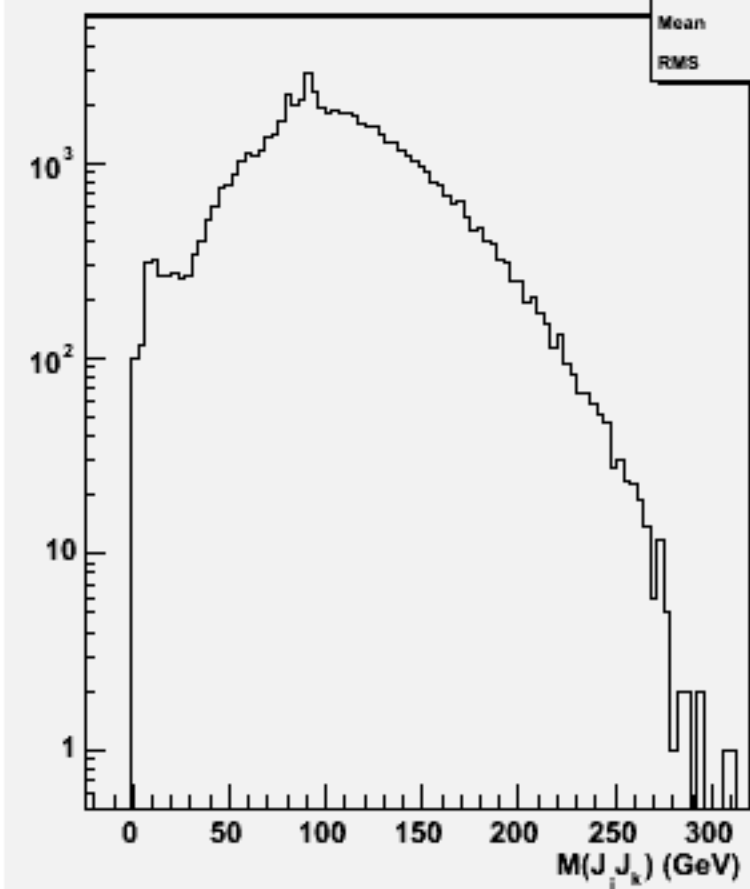
2jets mass(All comb)w103126 e1a_n1sssc_o
