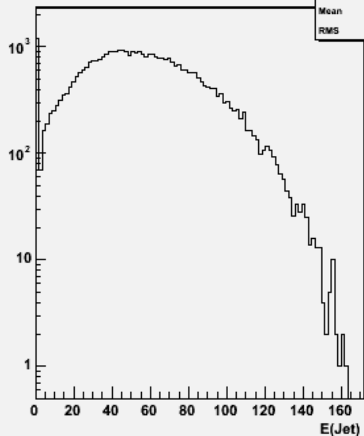
Jet energies(All jets)w103114 e1a_n1sse2n2_o
