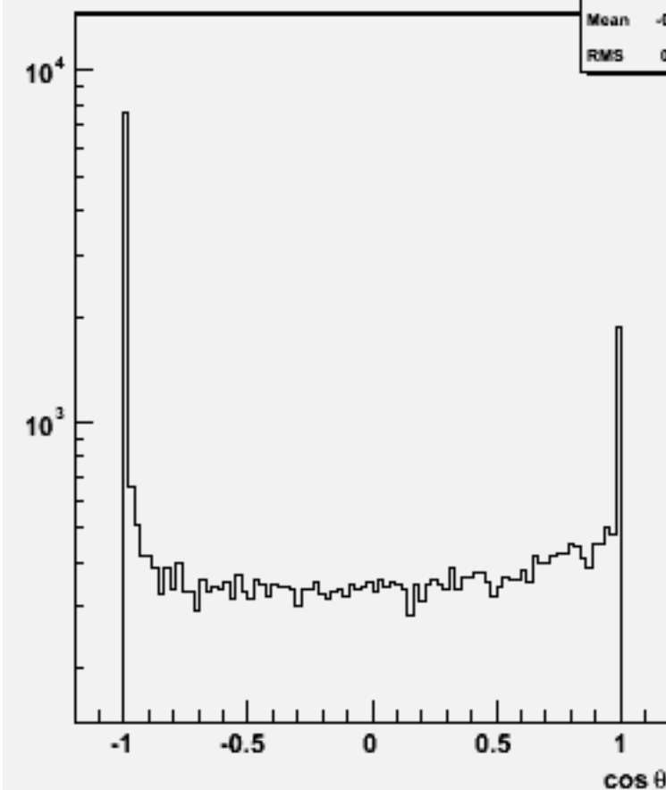
Jet cos \theta (All jets)w103114 e1a_n1sse2n2_o
