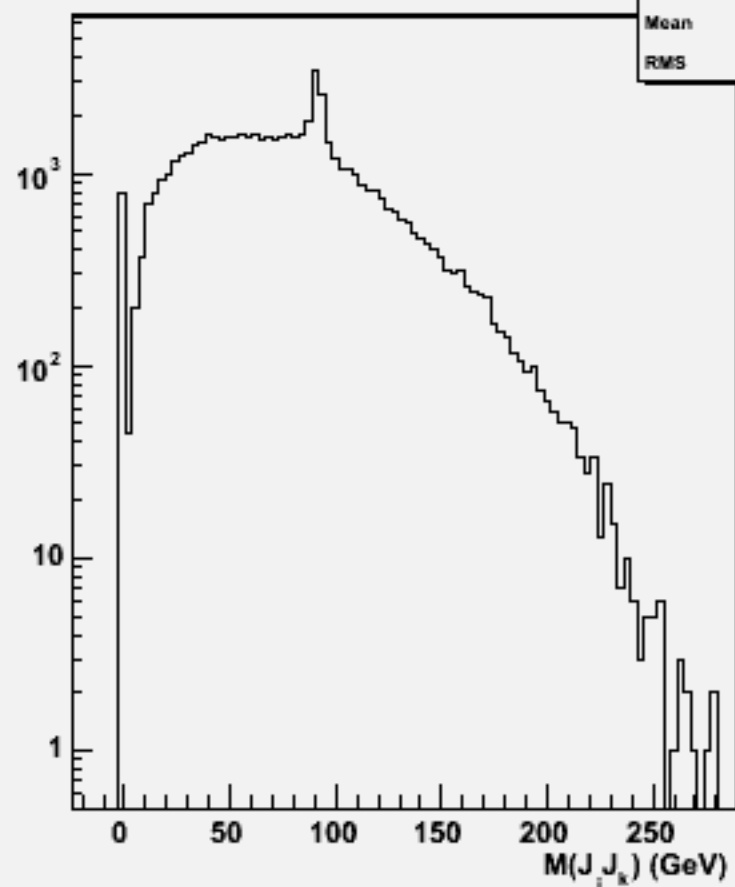
2jets mass(All comb)w103114 e1a_n1sse2n2_o
