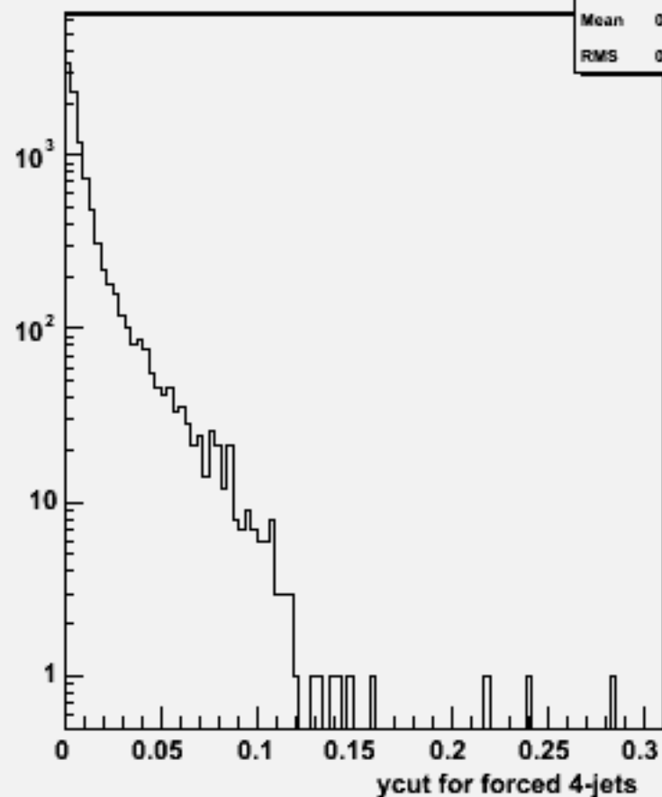
Ycut for 4-jets :w103114 e1a_n1sse2n2_o
