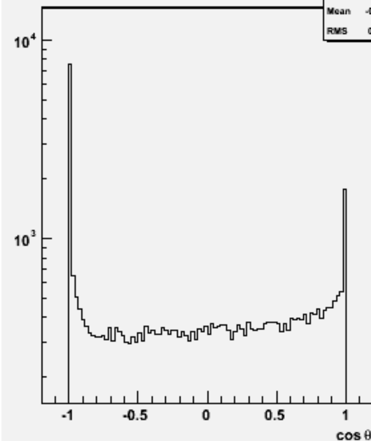
Jet cos \theta (All jets)w103098 e1a_n1dde3n3_o
