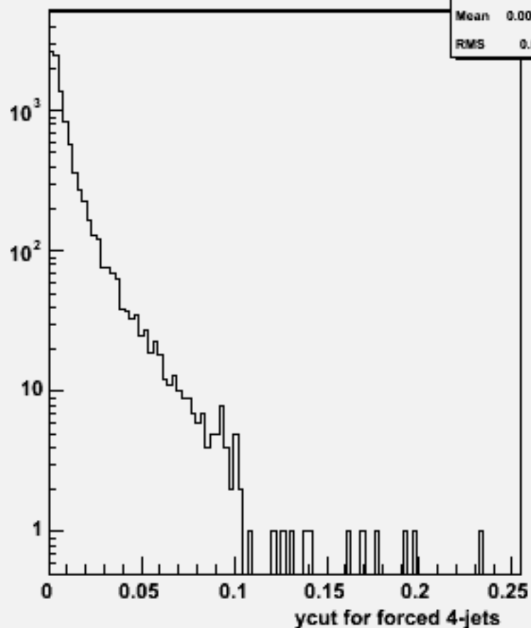
Ycut for 4-jets :w103098 e1a_n1dde3n3_o
