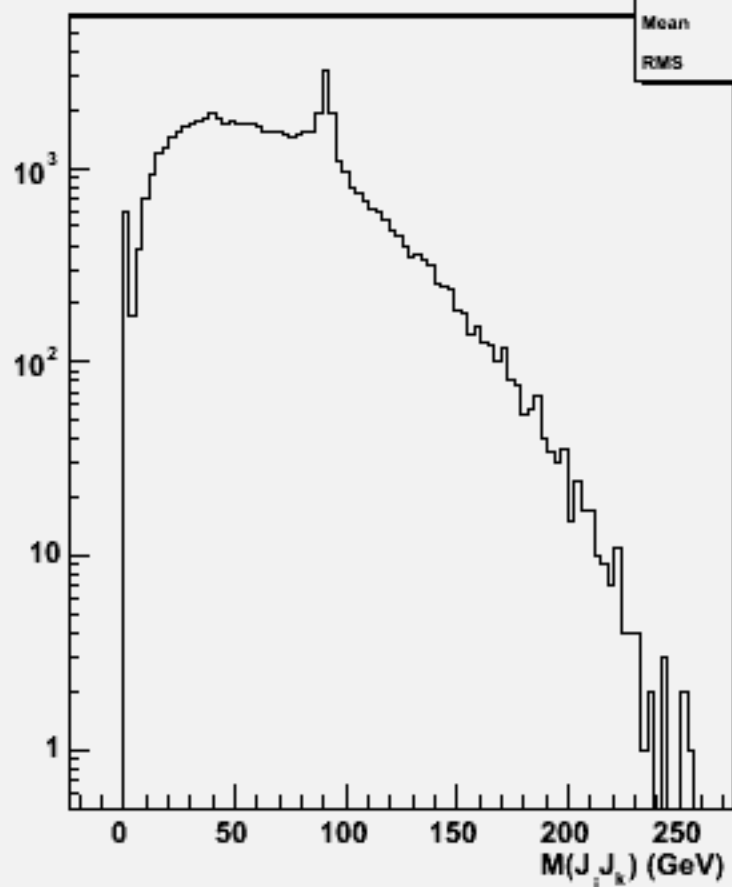
2jets mass(All comb)w103098 e1a_n1dde3n3_o
