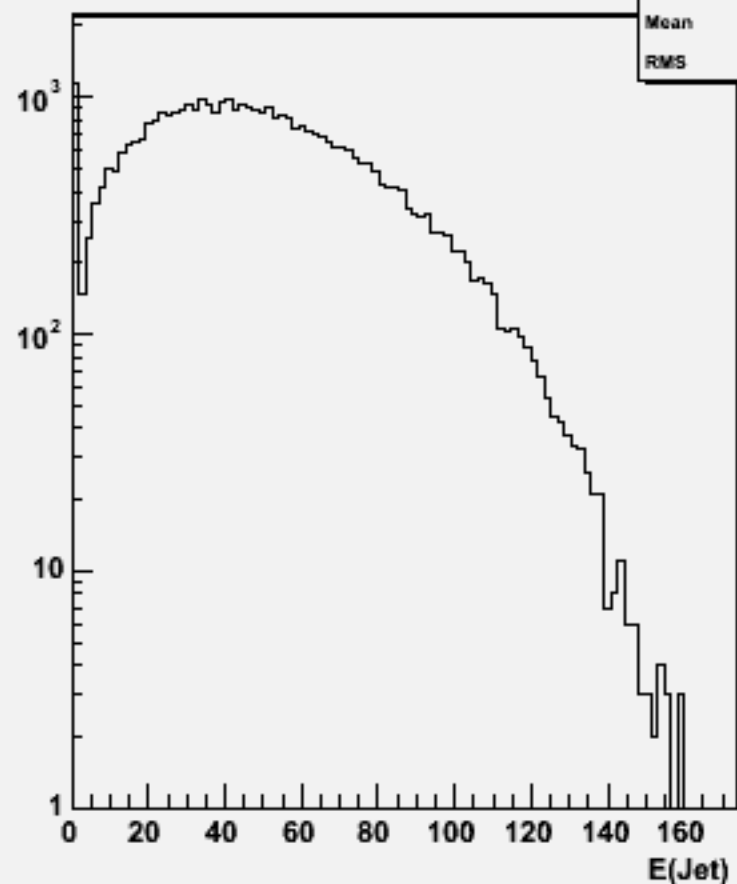
Jet energies(All jets)w103098 e1a_n1dde3n3_o
