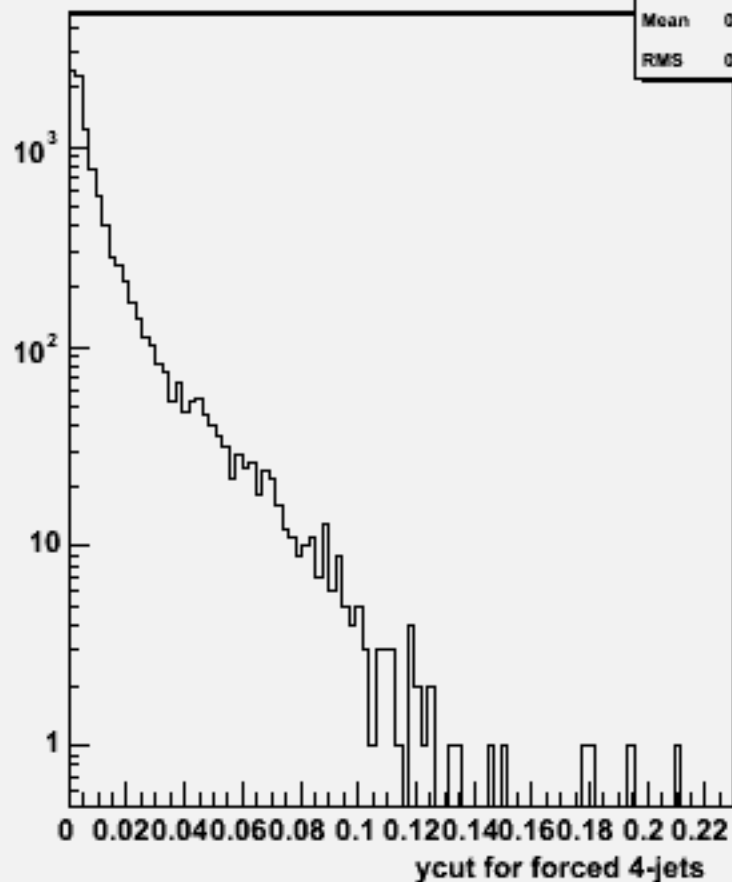
Ycut for 4-jets :w103094 e1a_n1dde2n2_o
