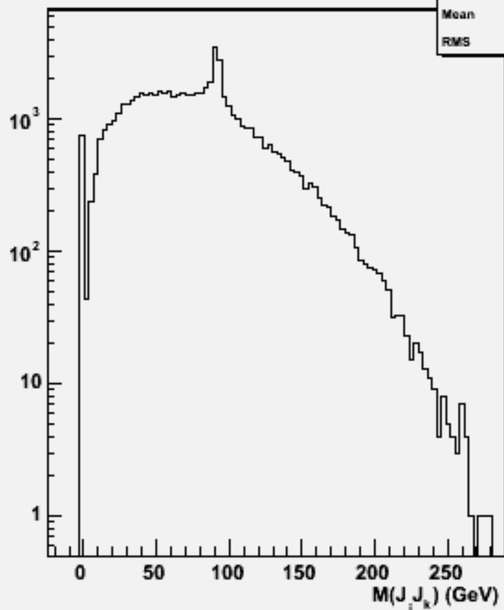
2jets mass(All comb)w103094 e1a_n1dde2n2_o
