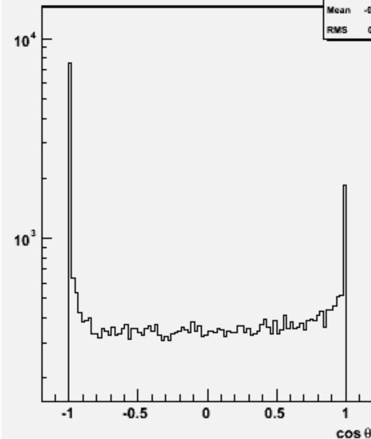
Jet cos \theta (All jets)w103094 e1a_n1dde2n2_o
