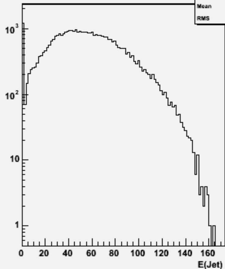
Jet energies(All jets)w103094 e1a_n1dde2n2_o
