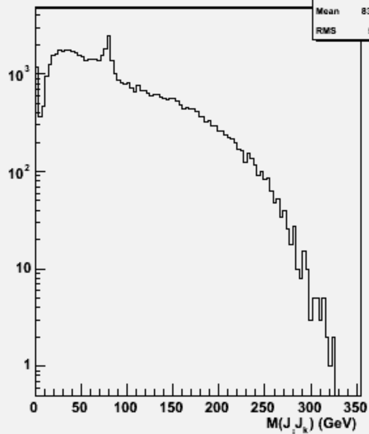
2jets mass(All comb)w103087 e1a_n1e3e3sc_o
