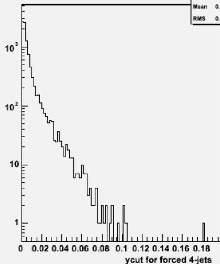
Ycut for 4-jets :w103087 e1a_n1e3e3sc_o
