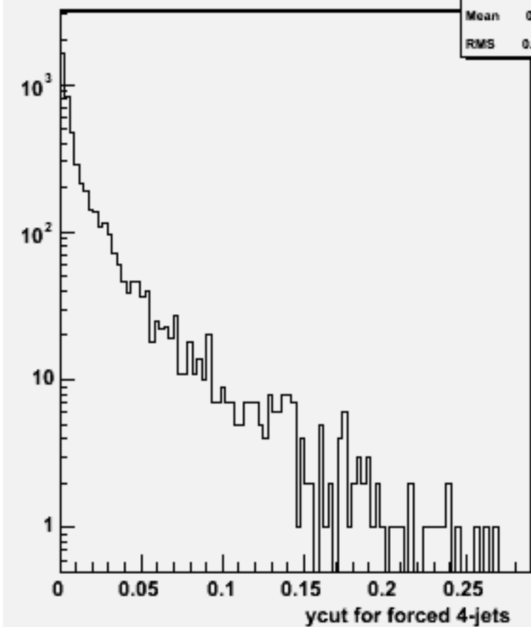
Ycut for 4-jets :w103070 e1a_n1e3e3e1n1_o
