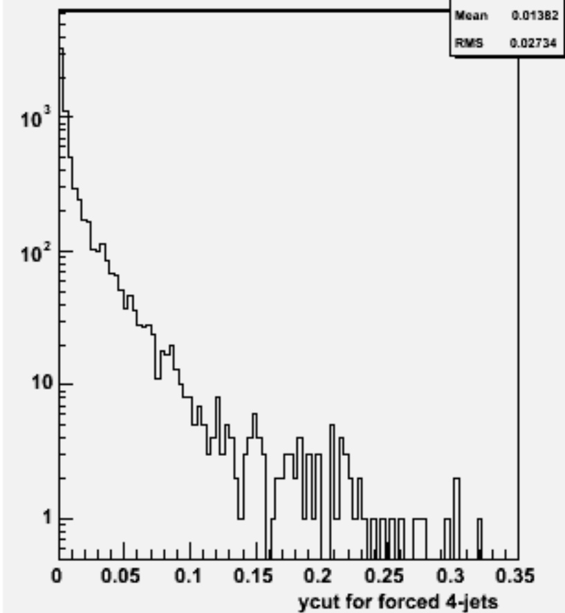
Ycut for 4-jets :w103054 e1a_n1e2e2n2_o
