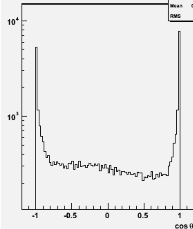
Jet cos \theta (All jets)w103048 e1a_n1e1e1sc_o
