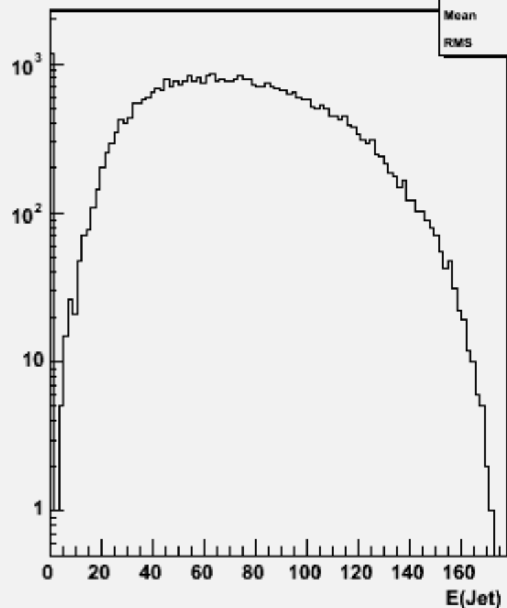
Jet energies(All jets)w103048 e1a_n1e1e1sc_o
