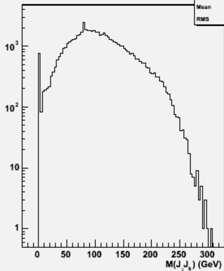
2jets mass(All comb)w103048 e1a_n1e1e1sc_o
