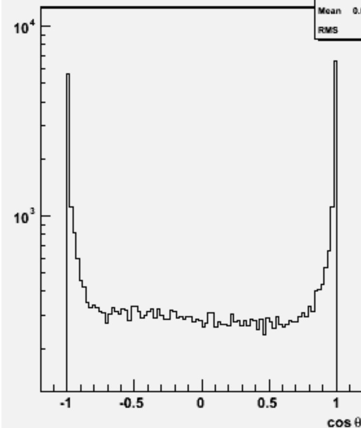
Jet cos \theta (All jets)w103046 e1a_n1e1e1sc_o
