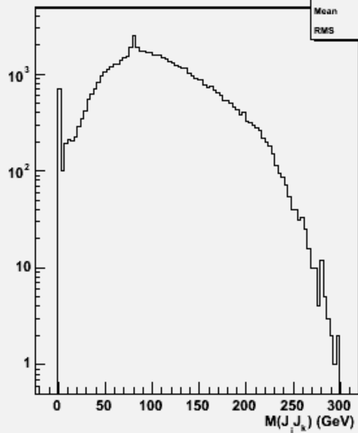
2jets mass(All comb)w103046 e1a_n1e1e1sc_o
