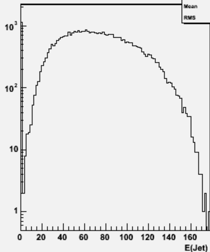
Jet energies(All jets)w103046 e1a_n1e1e1sc_o
