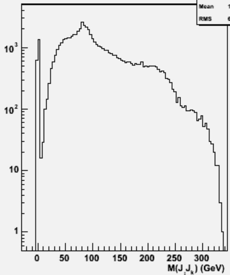
2jets mass(All comb)w103045 e1a_n1e1e1du_o
