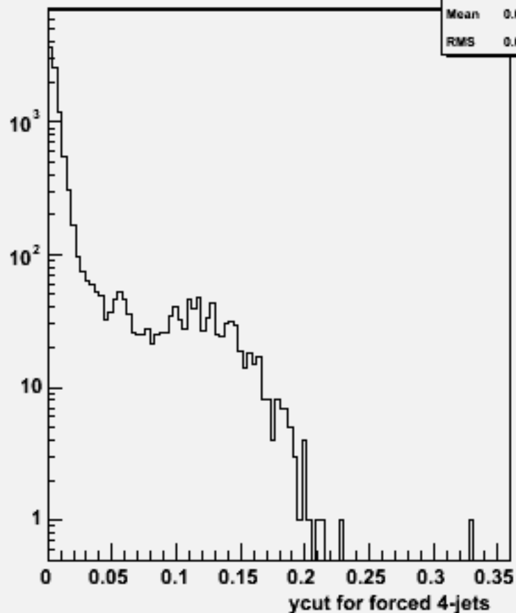
Ycut for 4-jets :w103045 e1a_n1e1e1du_o
