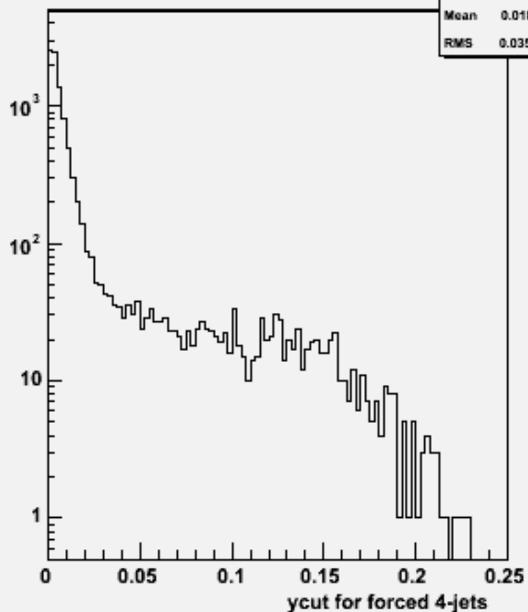
Ycut for 4-jets :w103043 e1a_n1e1e1du_o
