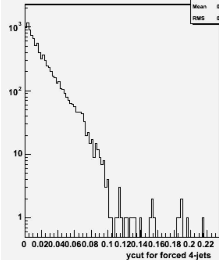
Ycut for 4-jets :w103040 e1a_n1e1e1e3n3_o
