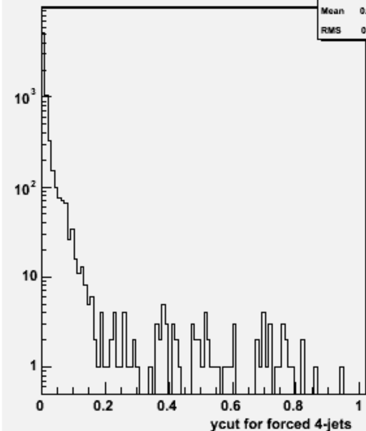
Ycut for 4-jets :w103039 e1a_n1e1e1e3n3_o
