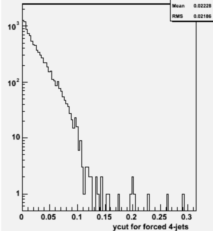
Ycut for 4-jets :w103034 e1a_n1e1e1e2n2_o
