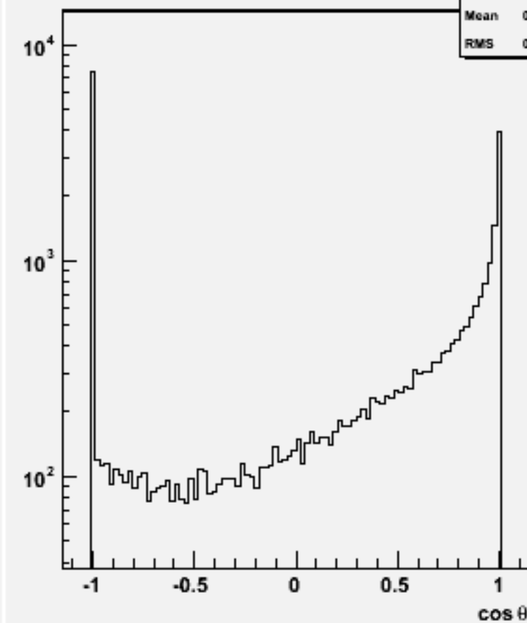
Jet cos \theta (All jets)w103031 e1a_n1e1e1e1n1_o
