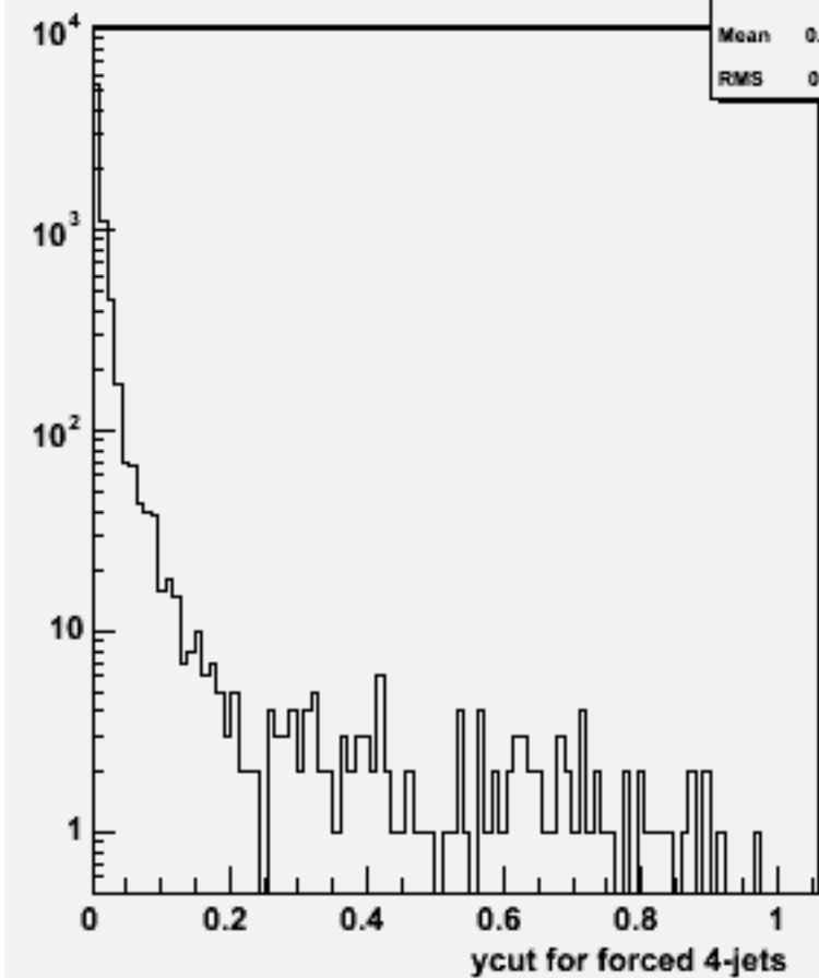
Ycut for 4-jets :w103031 e1a_n1e1e1e1n1_o
