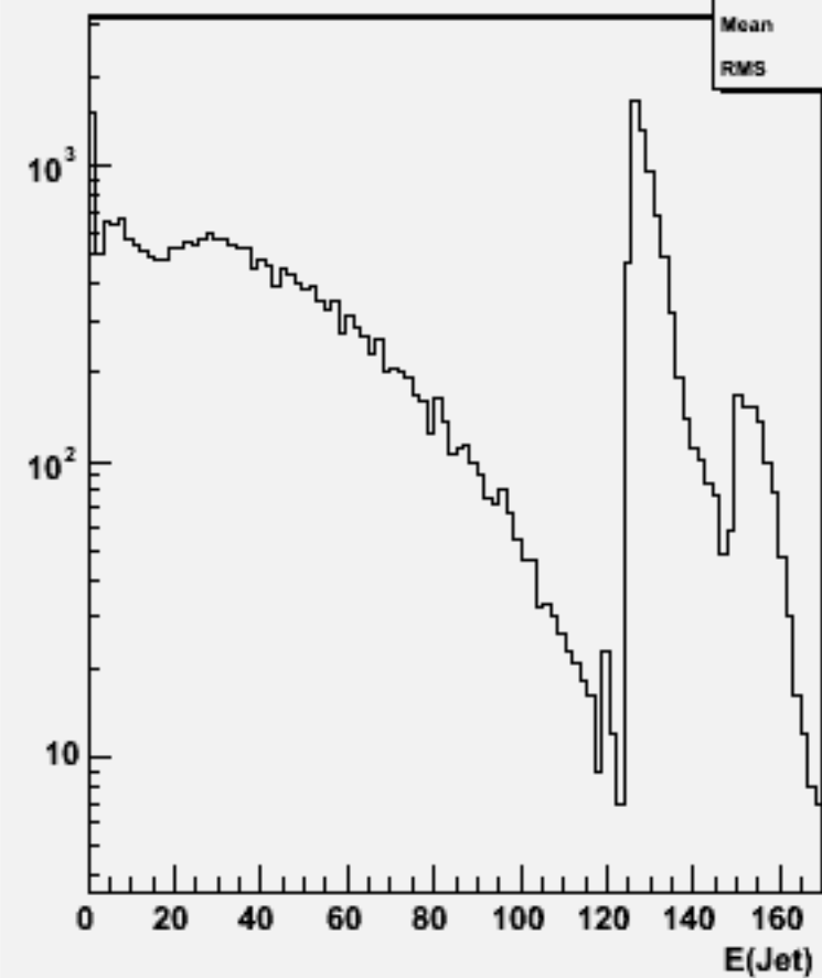
Jet energies(All jets)w103031 e1a_n1e1e1e1n1_o
