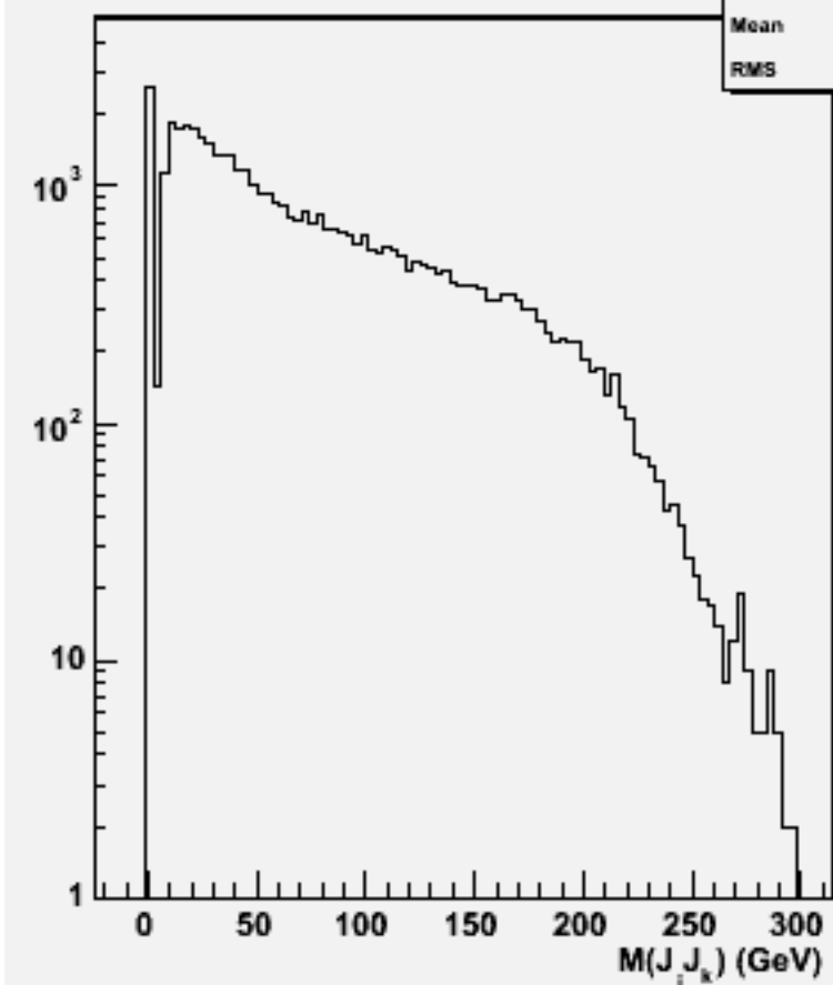
2jets mass(All comb)w103031 e1a_n1e1e1e1n1_o
