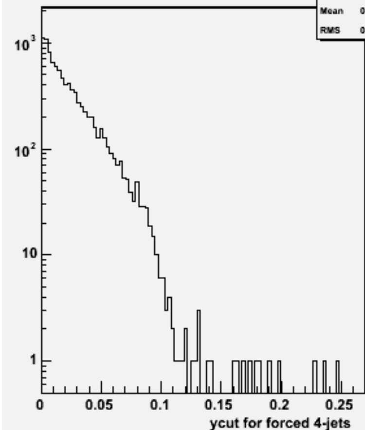
Ycut for 4-jets :w103030 e1a_n1e1e1n1_o
