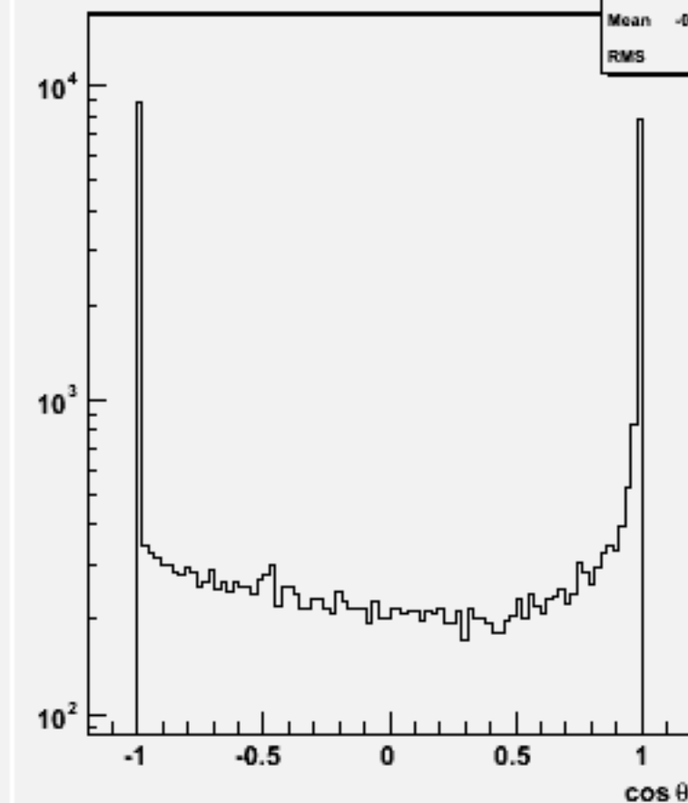
Jet cos \theta (All jets)w103030 e1a_n1e1e1n1_o
