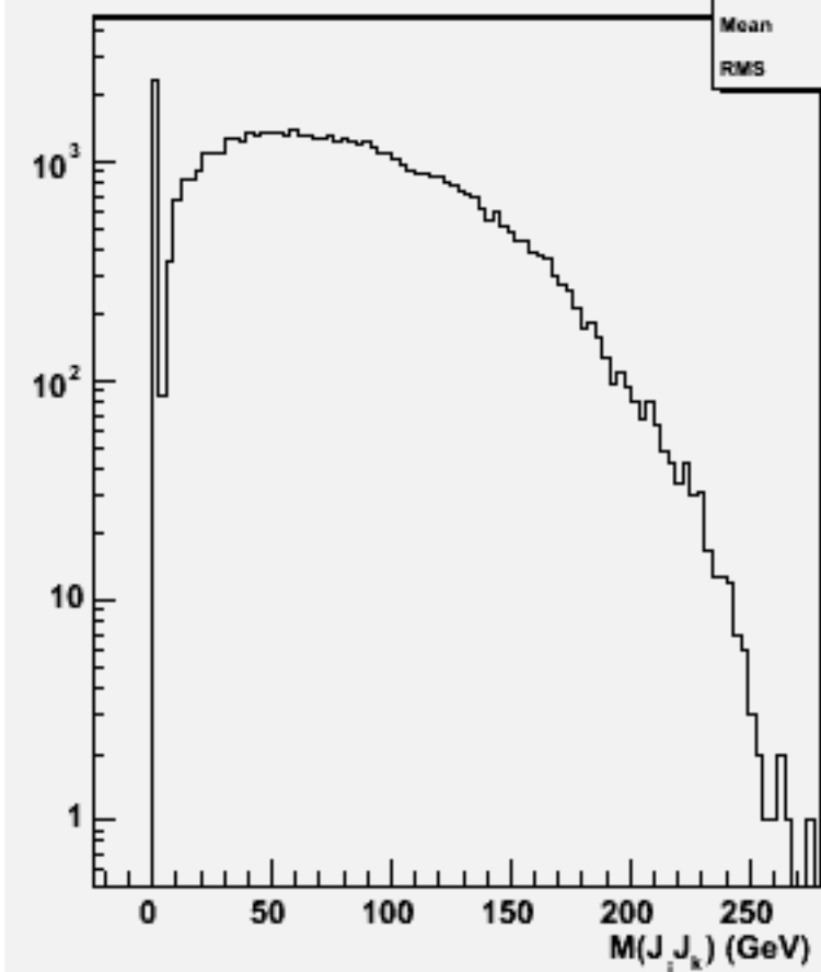
2jets mass(All comb)w103030 e1a_n1e1e1n1_o
